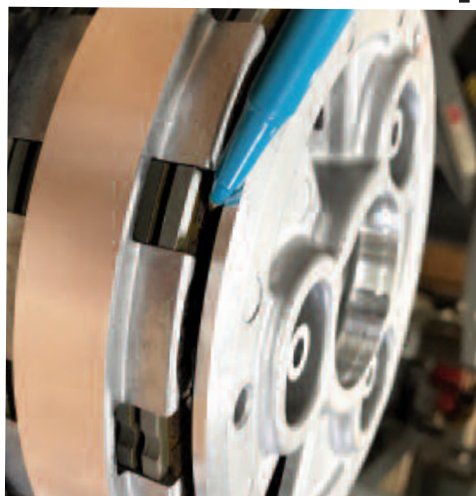
Photo #2. Not seated - see gap. Clutch will not work. Install friction steel friction on the pressure plate and hold as one unit while sliding on to locate teeth on the inner hub. They must mesh and sit flat like in Photo #1.
