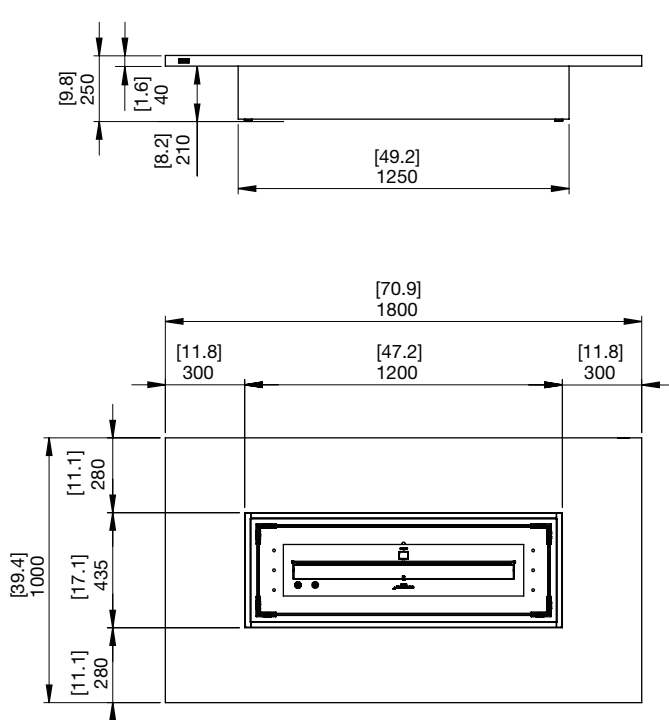
Line drawings show concrete models without a Fire Screen. Refer to the Fire Screen model specifications for dimensions.
