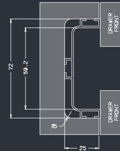
B. Centre Profile
