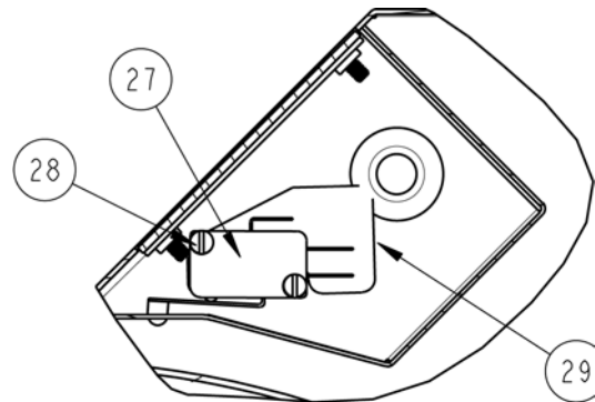
Fig 2: Detailed view of Safety Switch
