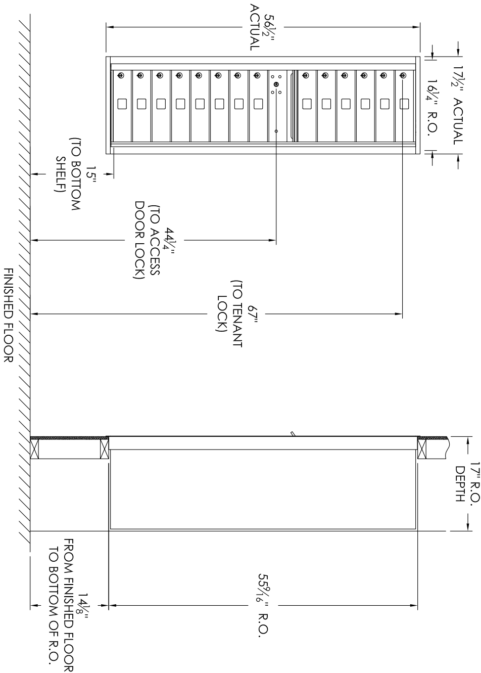
COMPARTMENT CHART
