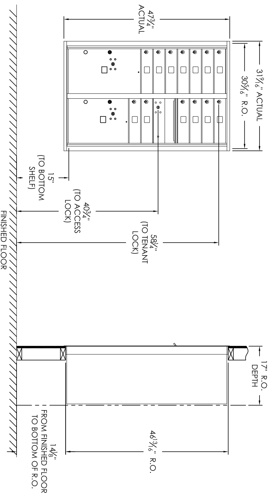
COMPARTMENT CHART
