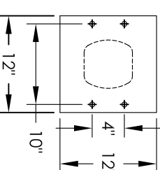
PEDESTAL DETAIL
