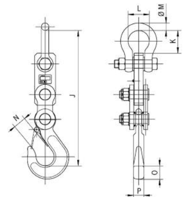
Load indicator. Model TZL/TZR with hook.
