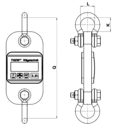
Load indicator. Model TZL/TZR with shackle.
