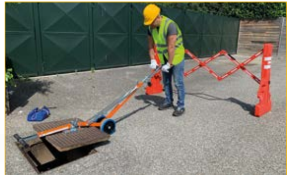
Use 2: opening with wheeled lever APS90 or APS80.
