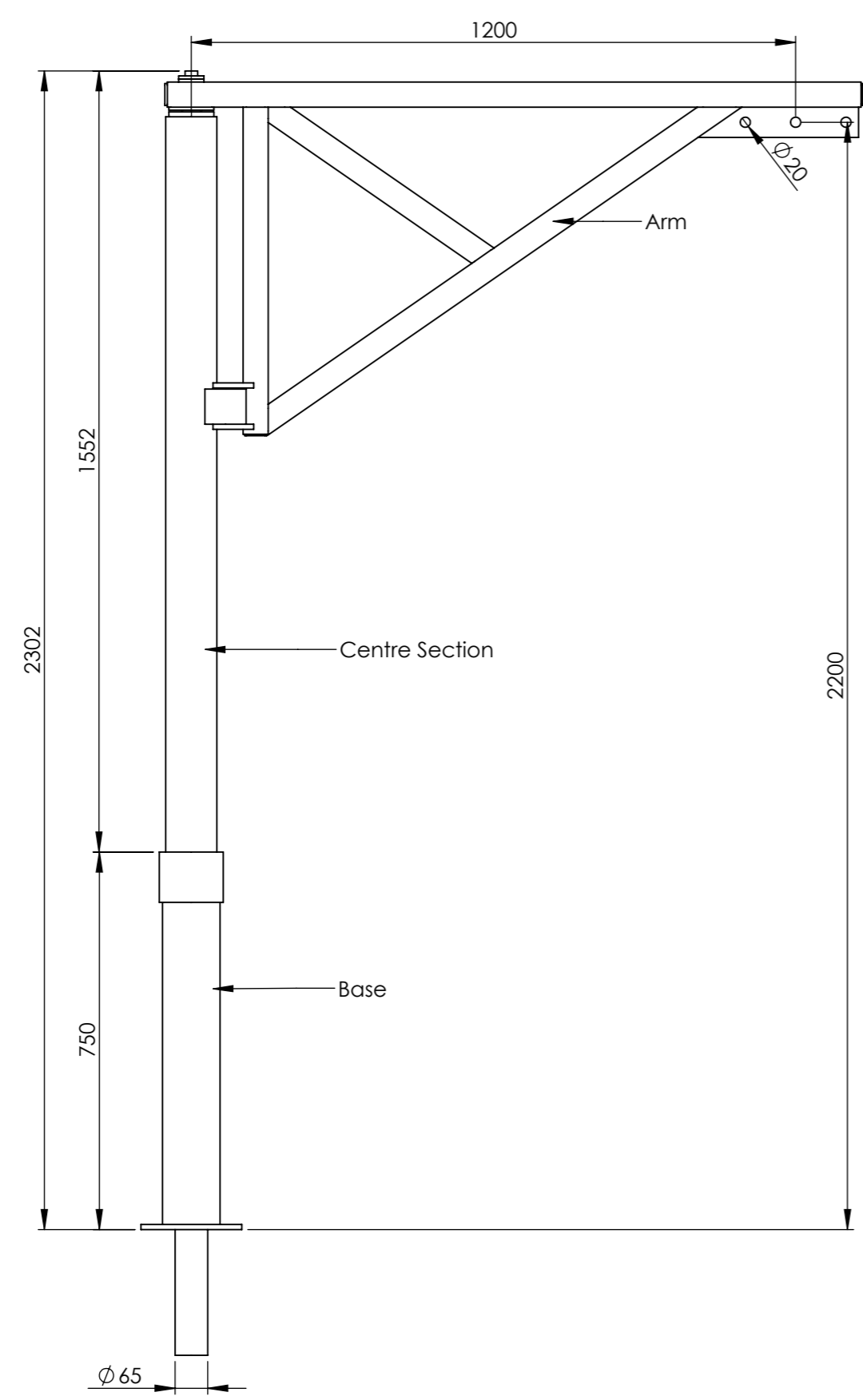
Front Elevation
