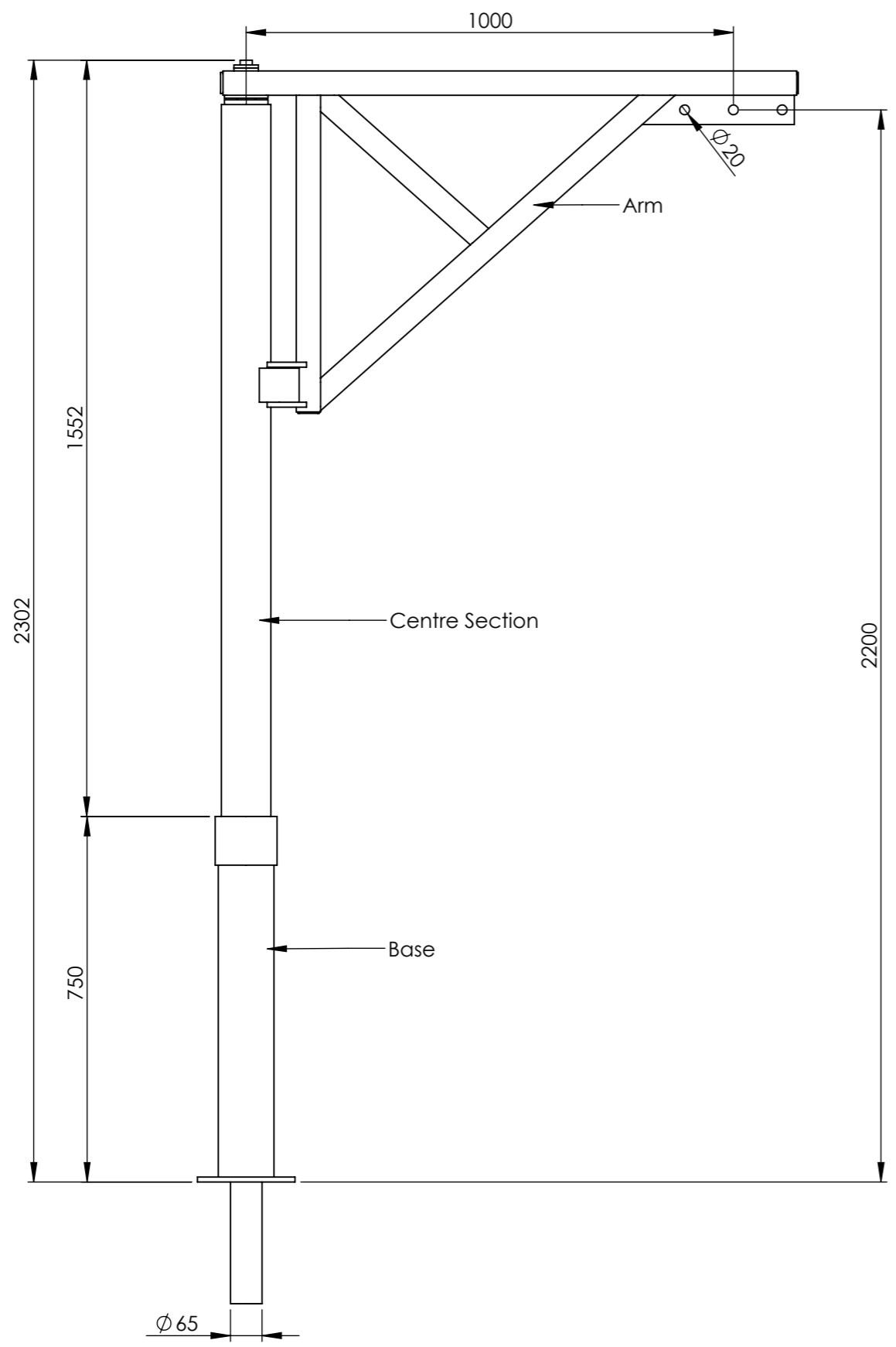
Front Elevation
