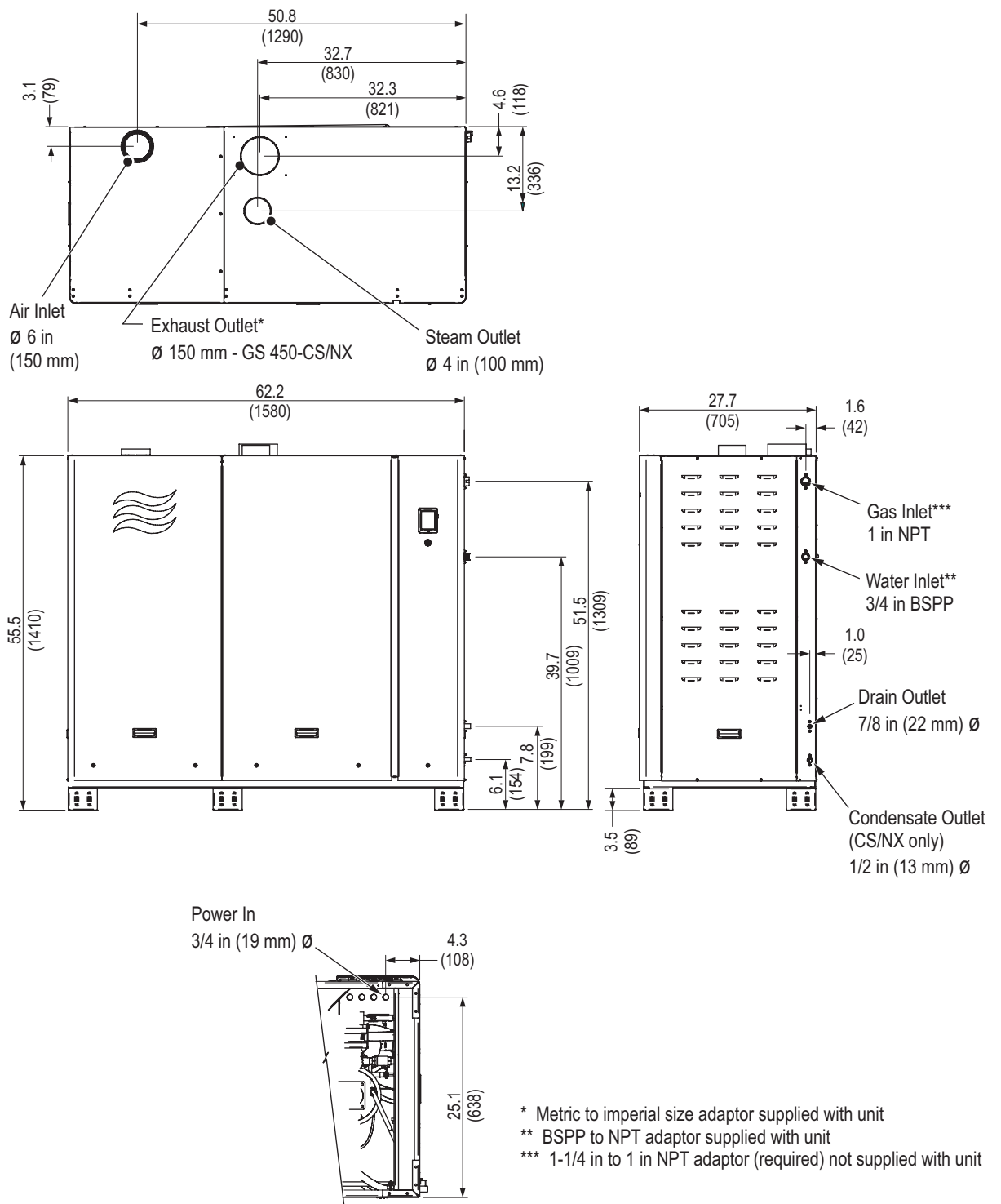
Figure 39: Nortec GS 450
