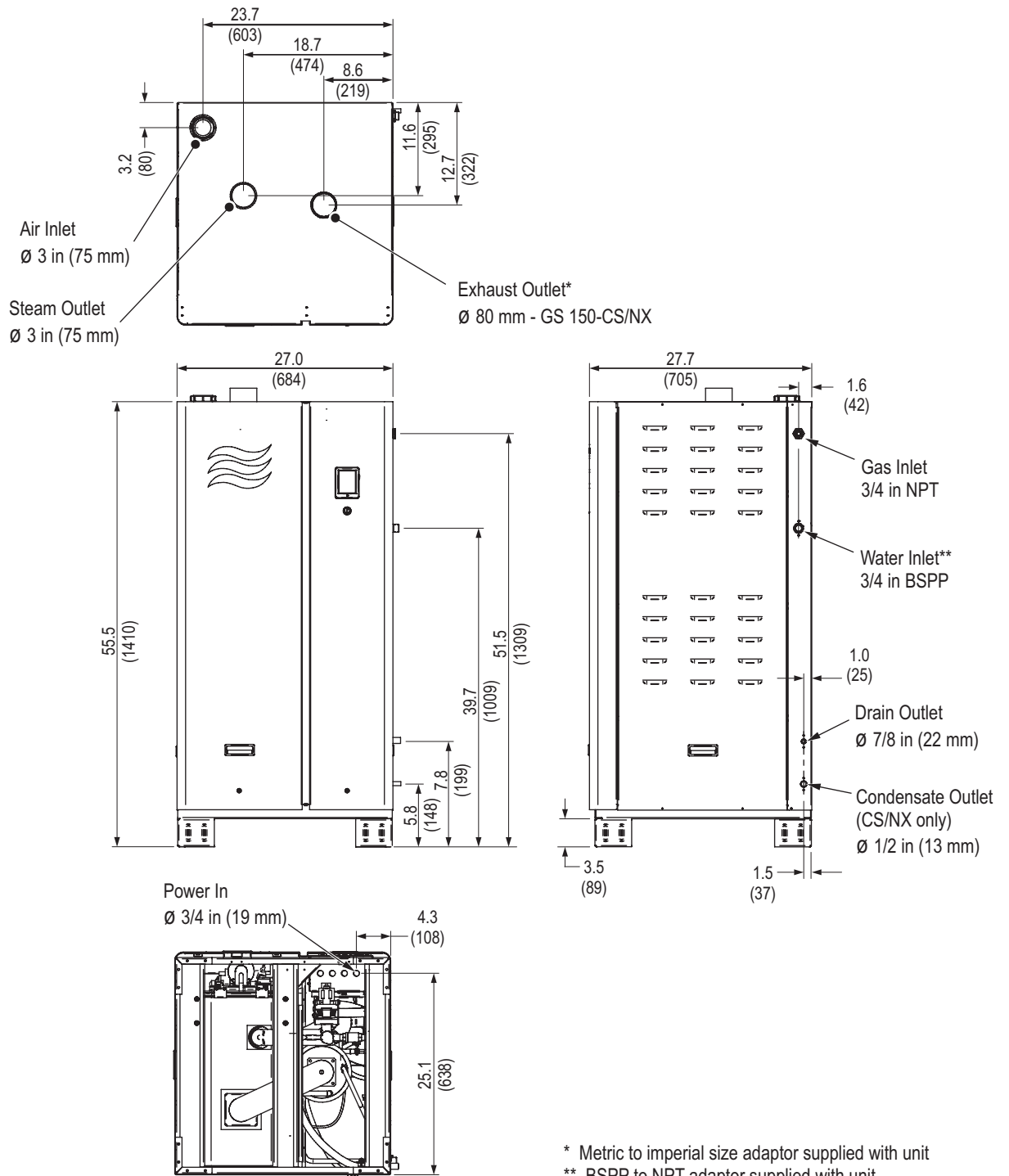
Figure 37: Nortec GS 150
