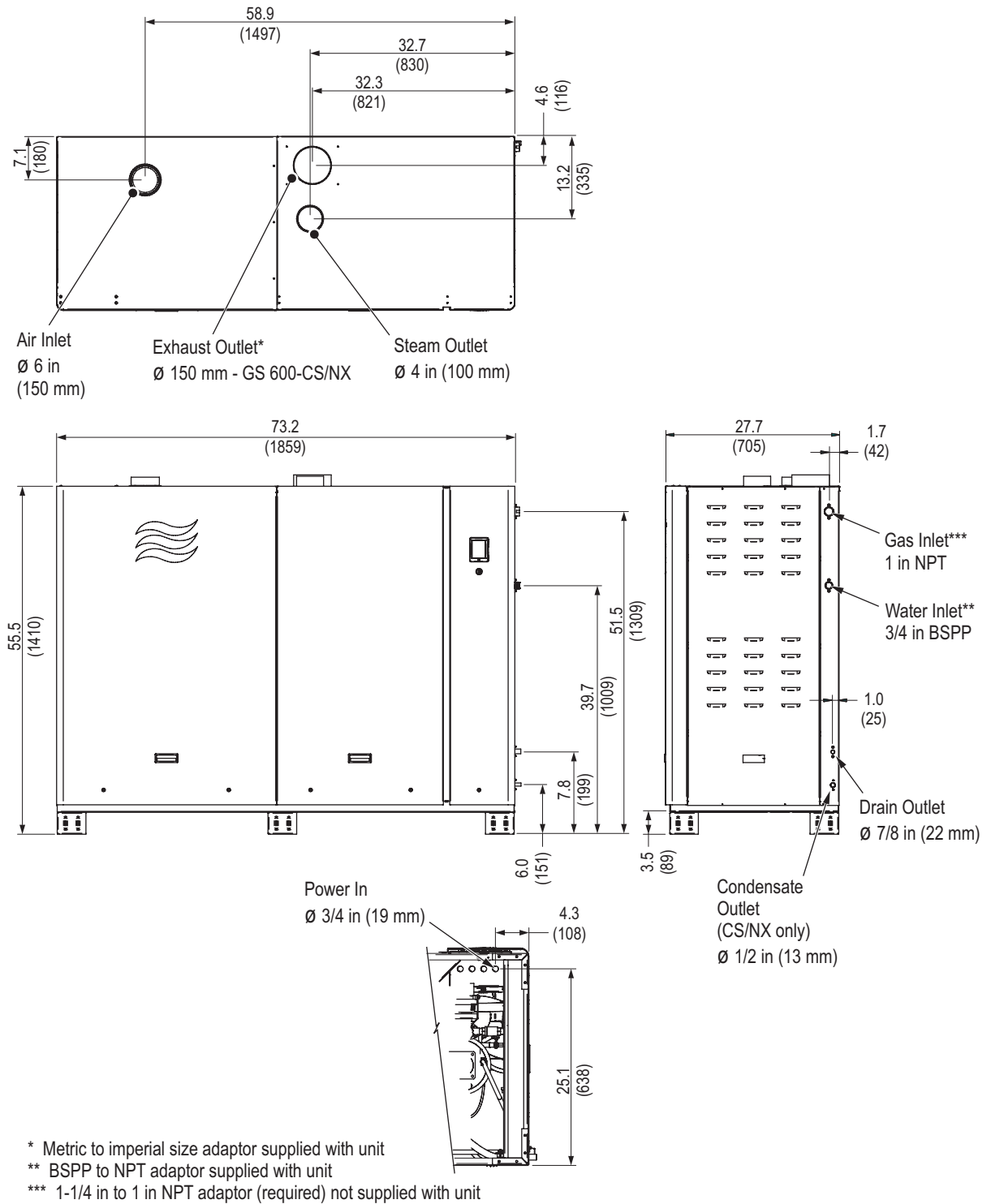
Figure 40: Nortec GS 600
