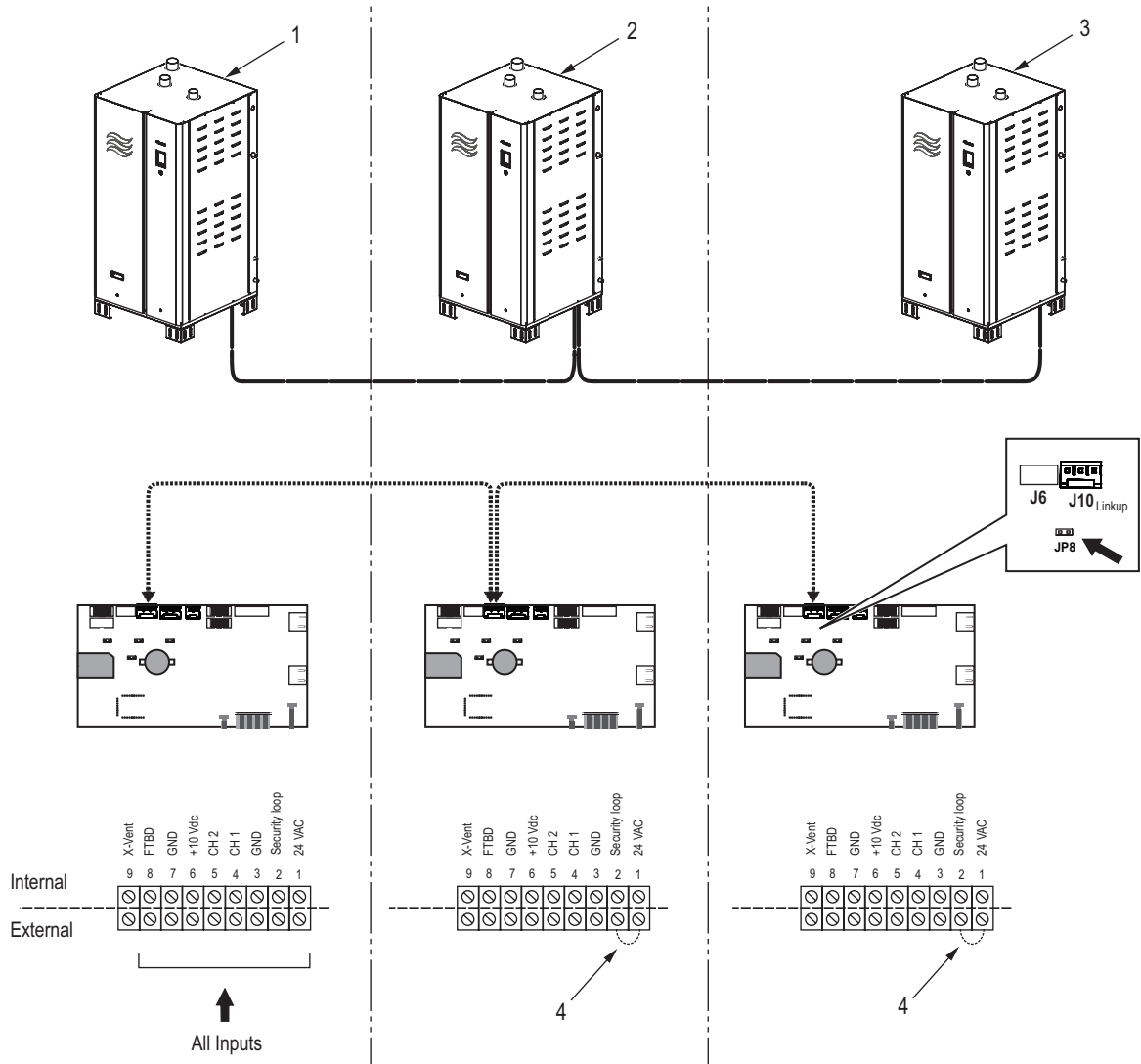
Figure 34: Multi-Unit Linkup Connections
