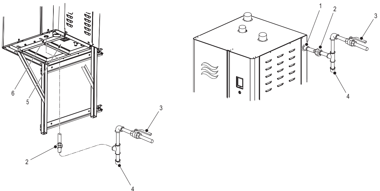
Figure 23: Gas Connection
