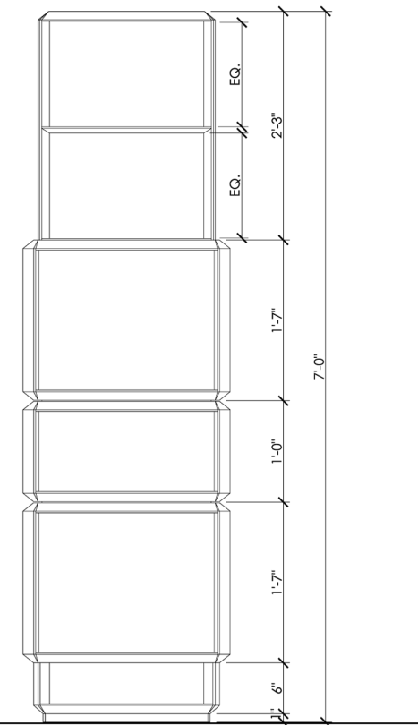
(UNIT ELEVATION) 24.5" x 24.5" x 84"(H)
