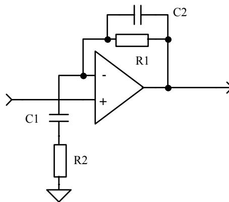
Figure 4.3 2 nd Stage Pre-emphasis Circuit
