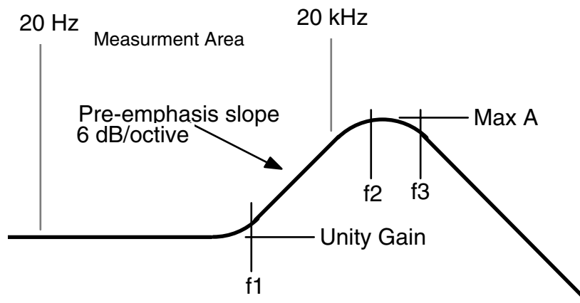
Figure 4.2 Pre-emphasis Curve
