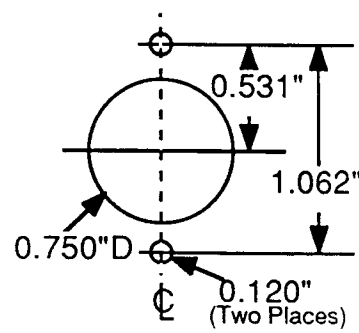
Fig 3.1 Switchcraft D3M Drill Template
