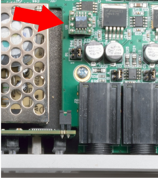
Figure 3 - Finished installation. White line on software chip must face the rear of the unit!
