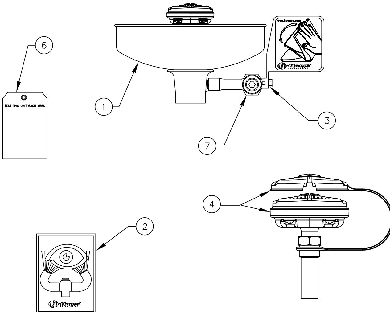
SP65 EYE/FACE WASH ASSEMBLY (INCLUDES: EYE/FACE WASH HEAD (SHOWN), EYEWASH HEAD (NOT SHOWN), EYEWASH FLOW CONTROL (NOT SHOWN), DUST COVER (SHOWN))
