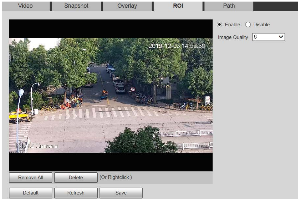
Figure 5-30 ROI settings
