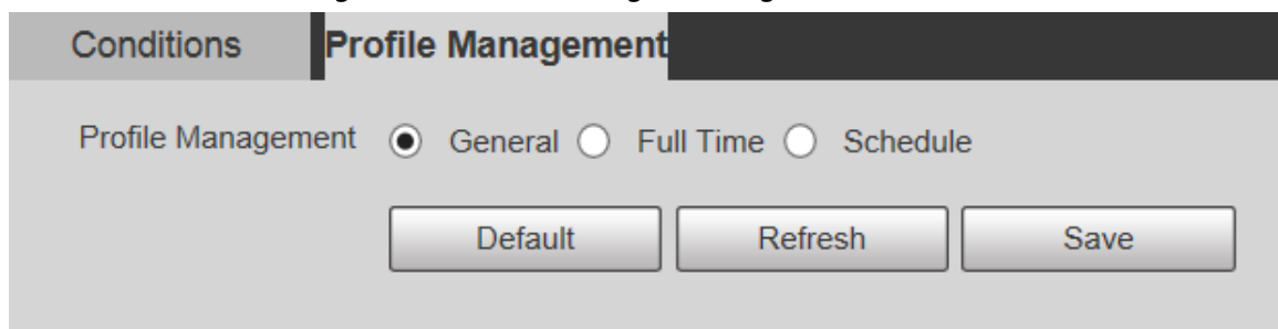
Figure 5-15 Profile management—general
