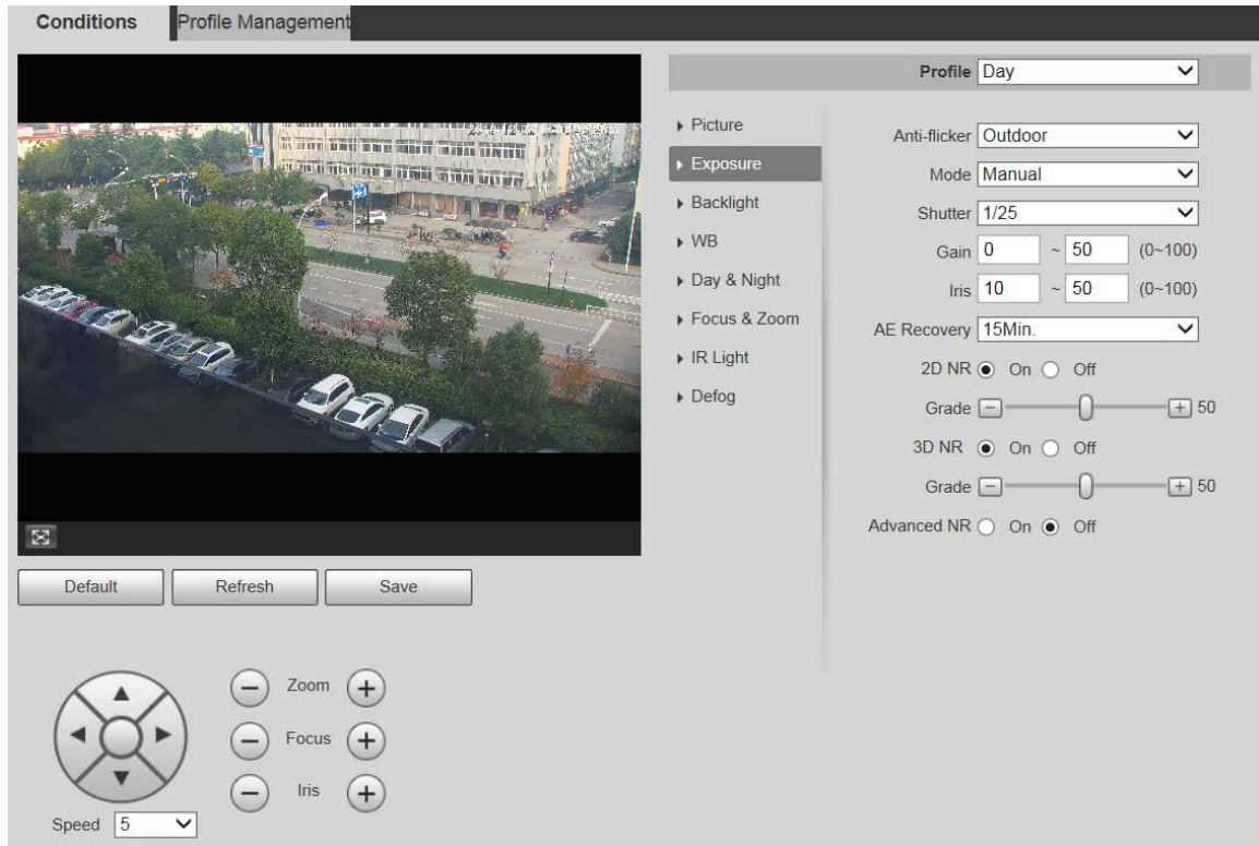
Figure 5-6 Exposure—manual mode
