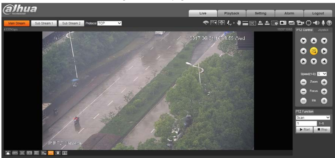
Figure 1-12 Live page
