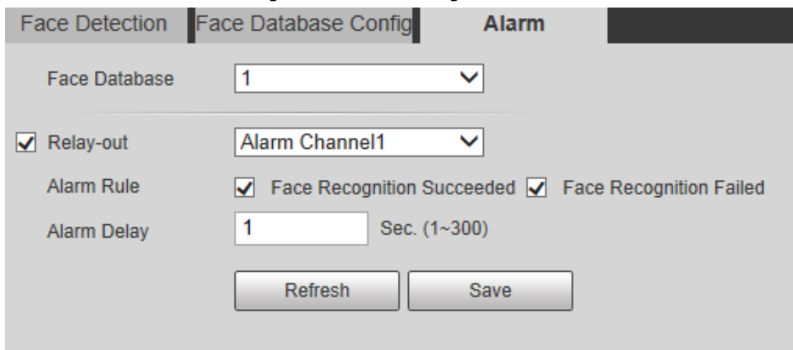
Figure 5-115 Alarm linkage
