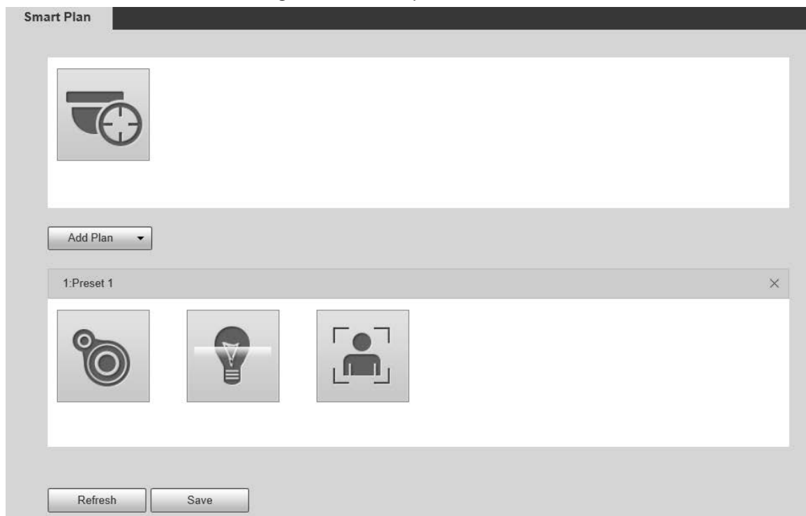
Figure 5-88 Smart plan (1)
