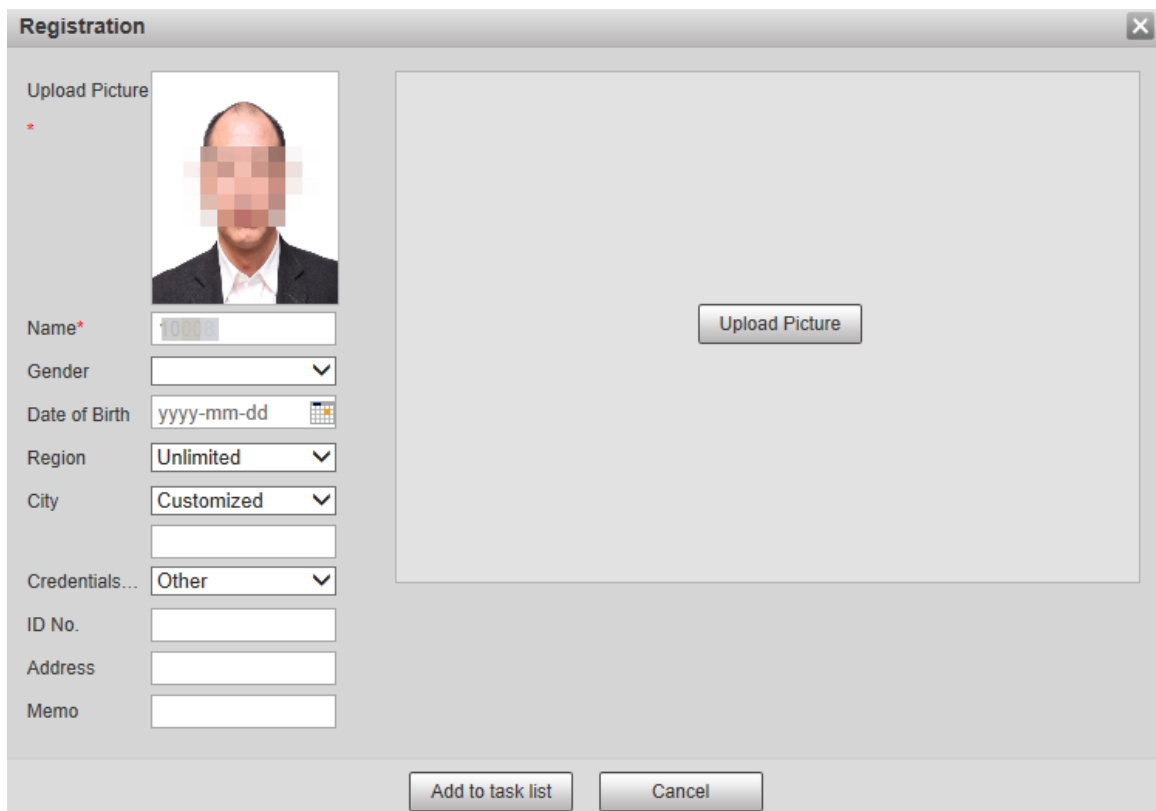
Figure 5-112 Registration page
