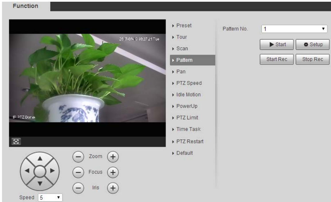
Figure 5-72 Pattern settings
