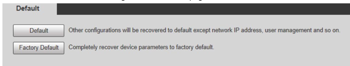
Figure 5-174 Default page
