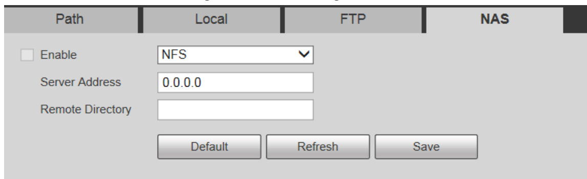
Figure 5-143 NAS settings
