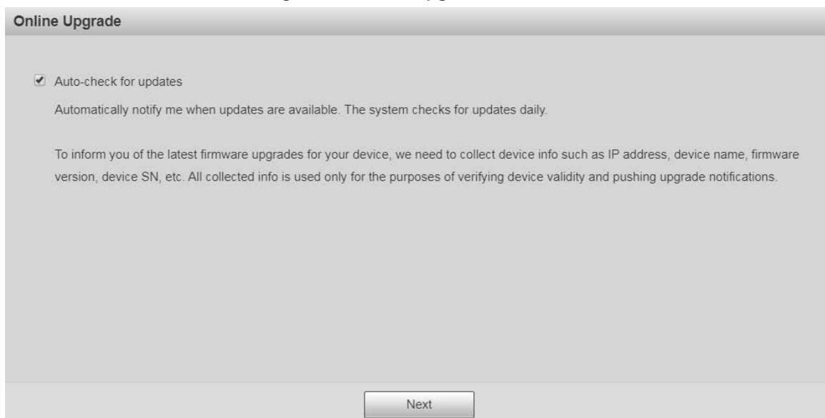
Figure 1-9 Online upgrade
