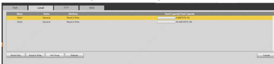
Figure 5-142 Local storage
