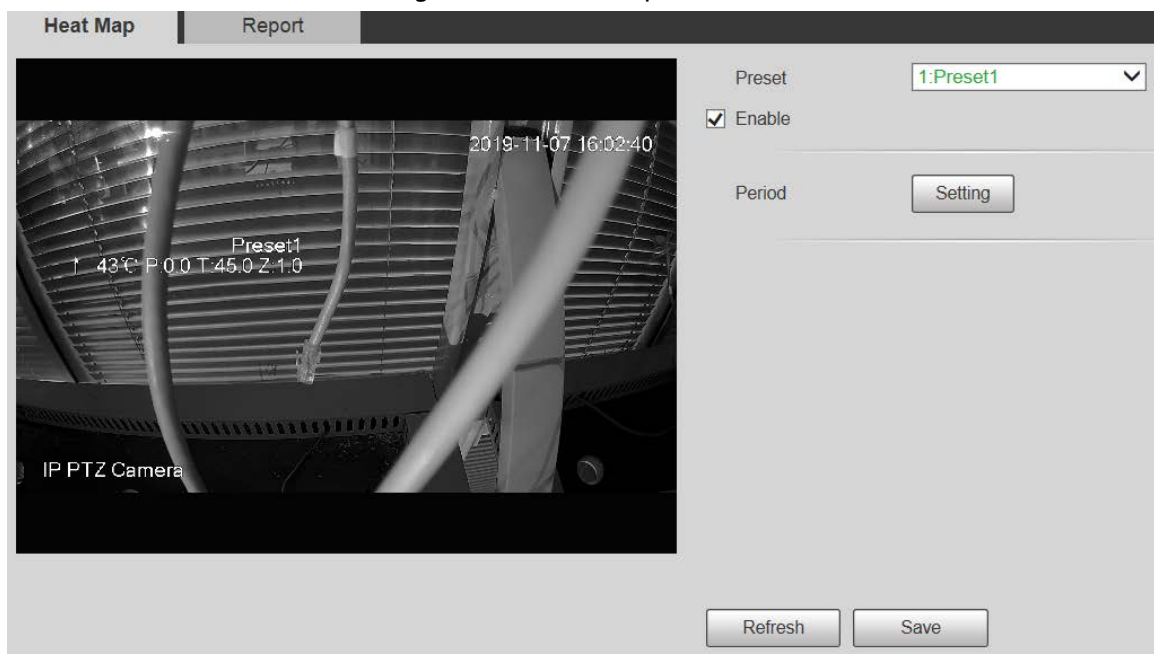
Figure 5-118 Heat map
