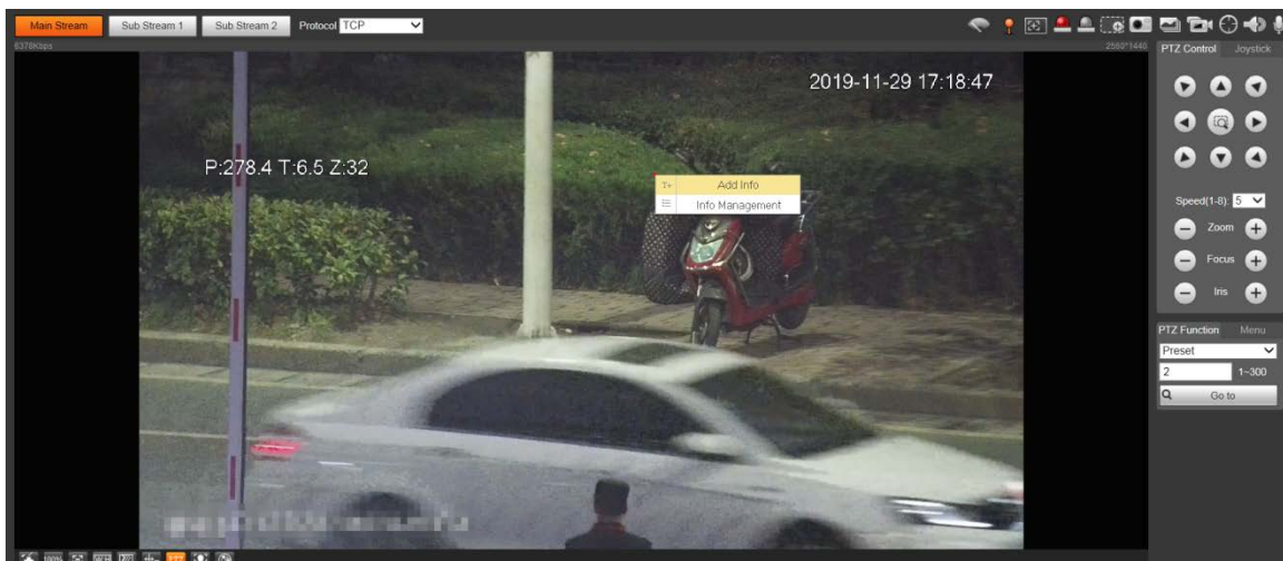
Figure 2-15 Mark—add comments
