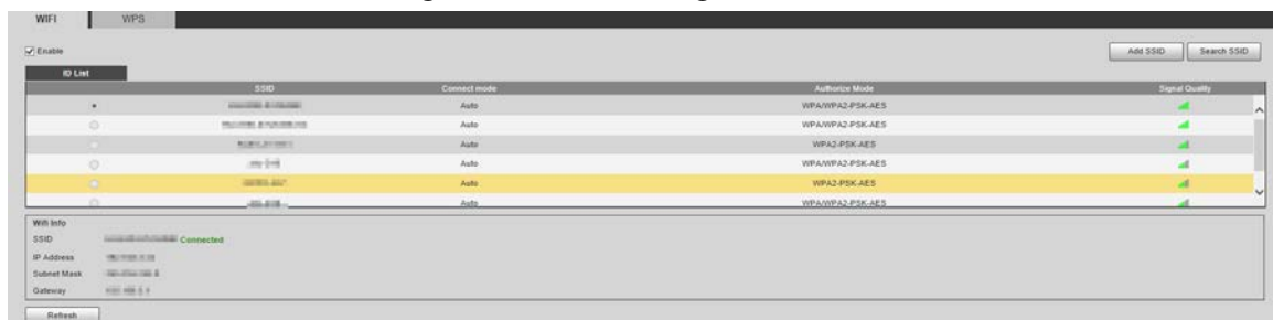
Figure 5-49 Wi-Fi settings (2)
