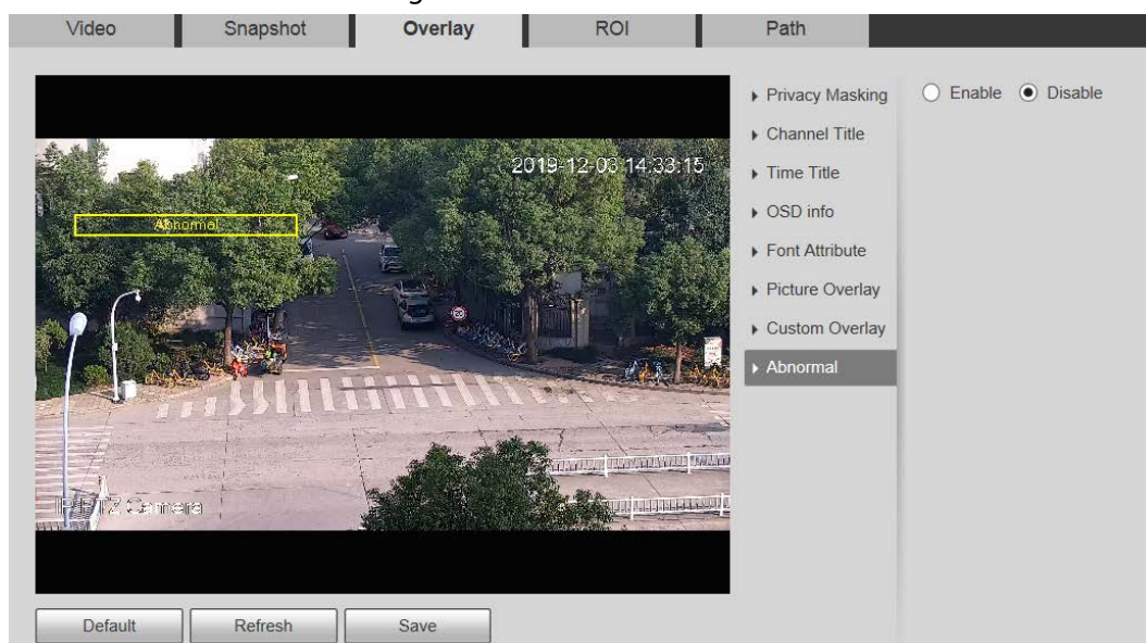
Figure 5-28 Abnormal
