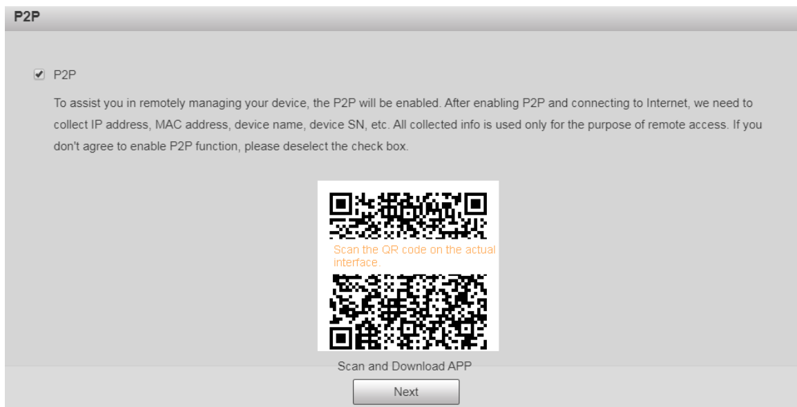
Figure 1-7 P2P page
