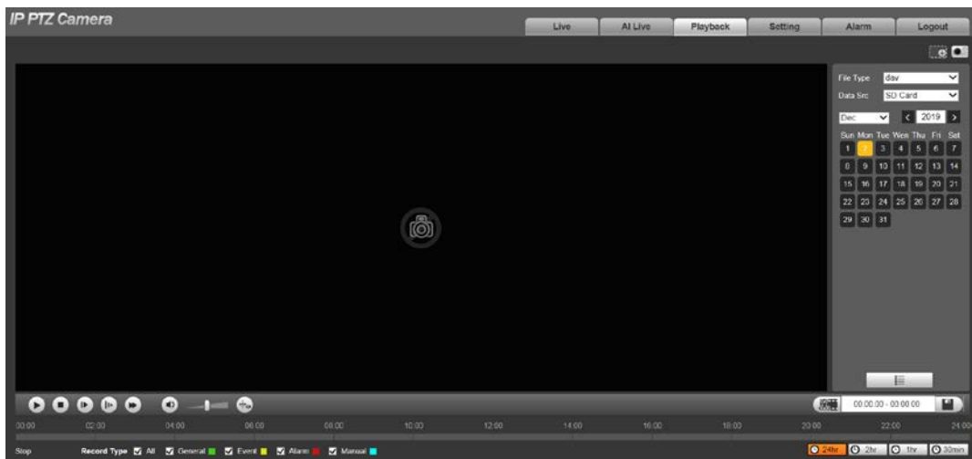
Figure 4-1 Playback page
