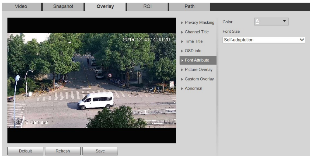
Figure 5-24 Font attribute
