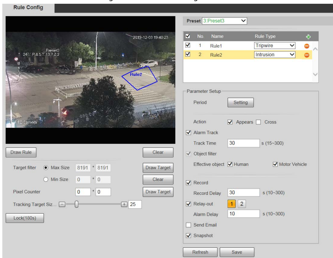
Figure 5-92 Intrusion settings
