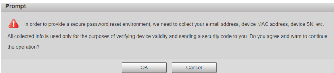
Figure 1-15 Prompt
