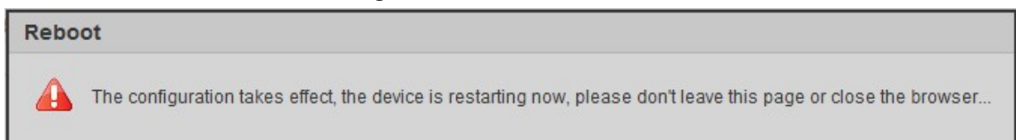
Figure 5-171 Reboot
