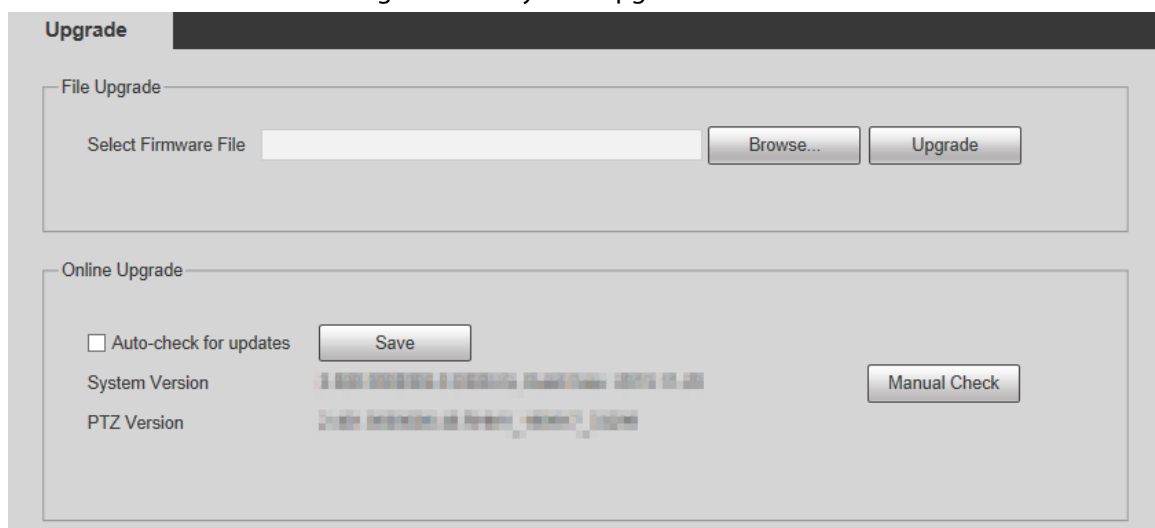
Figure 5-178 System upgrade
