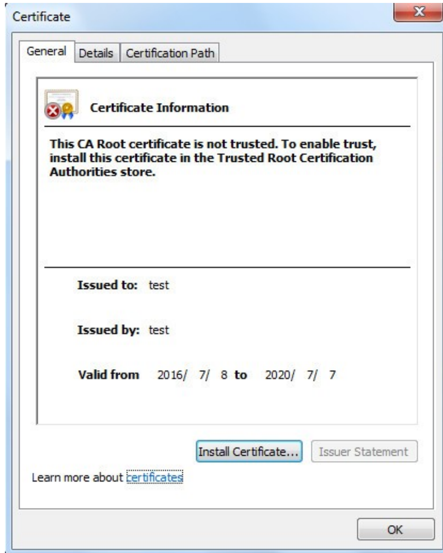
Figure 5-164 Certificate information
