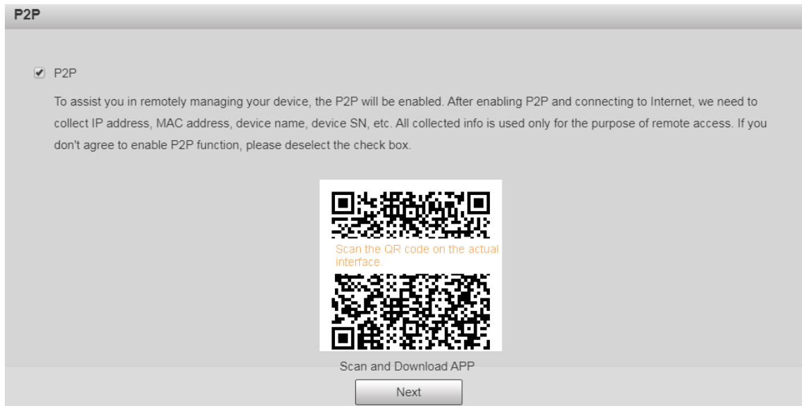
Figure 1-8 P2P page
