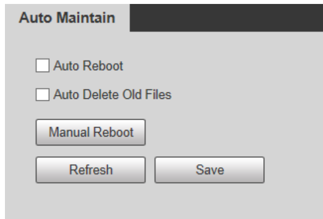
Figure 5-176 Auto maintain
