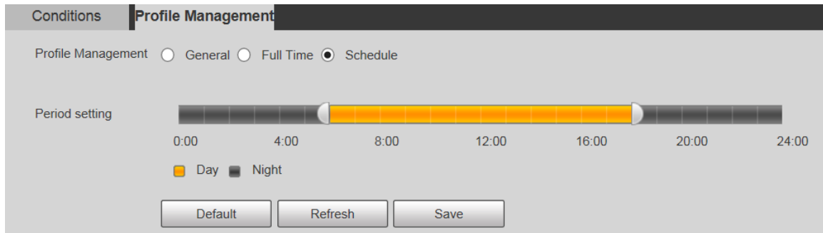
Figure 5-17 Profile management—schedule
