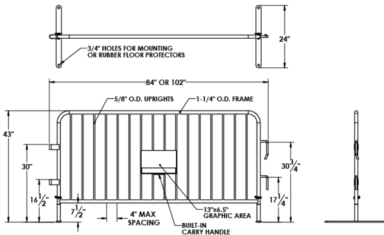
6.5' AND 8' STEEL BARRIERS FLAT FEET
