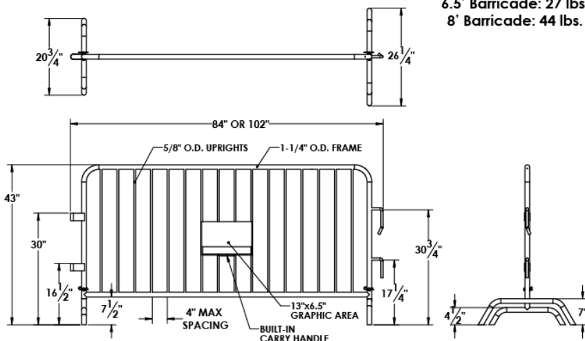
6.5' AND 8' STEEL BARRIERS BRIDGED FEET
