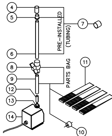
4 PIPE ASSEMBLY SCALE: NOT TO SCALE
