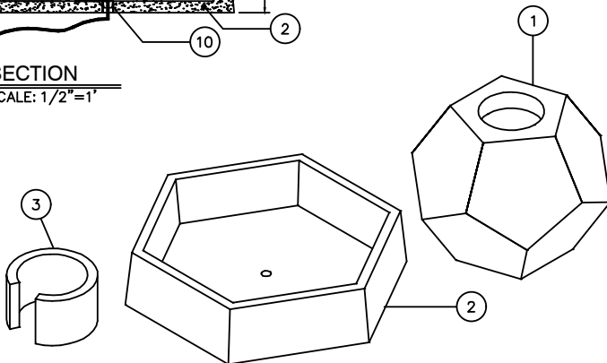
3 EXPLODED VIEW SCALE: 1/2"=1'
