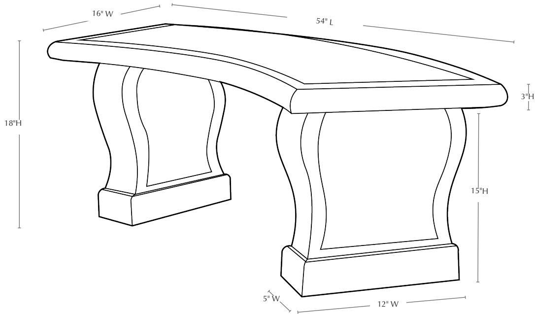
Isometric View
