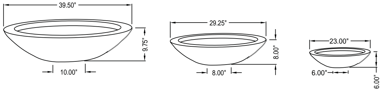
Isometric View
