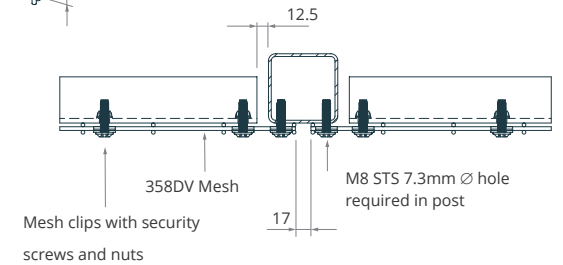
INGROUND POST
