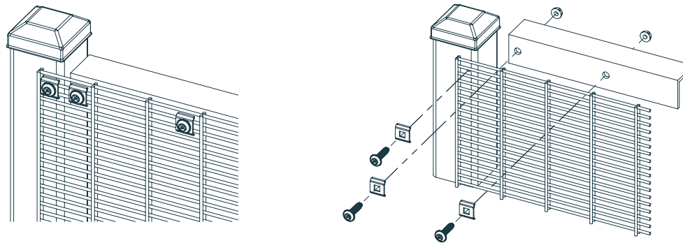
RAIL DETAIL
