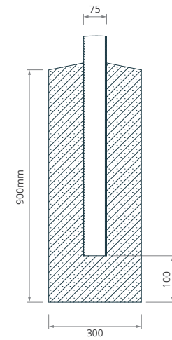
INGROUND POST
