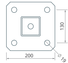
FLANGE POST
