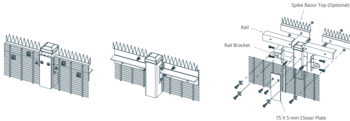
RAIL BRACKET DETAIL
