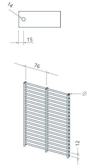
RAIL END DETAIL
