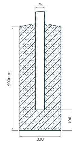
INGROUND POST
