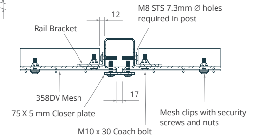
CONNECTION DETAIL
