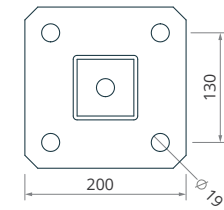
FLANGE POST
