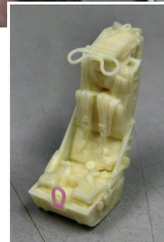
Assembled seat showing upper and lower ejection handles installed.
