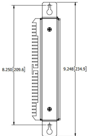
BACK VIEW (w/ Panel Mount Brackets)
