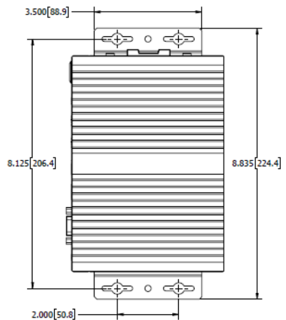
SIDE VIEW (w/ Shelf Mount Brackets)
