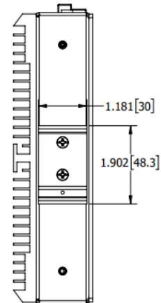
BACK VIEW (DIN Mount)
