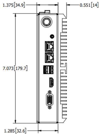
BACK VIEW (w/ Panel Mount Brackets)
