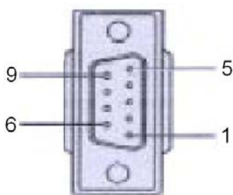
DB 9-pin Female
