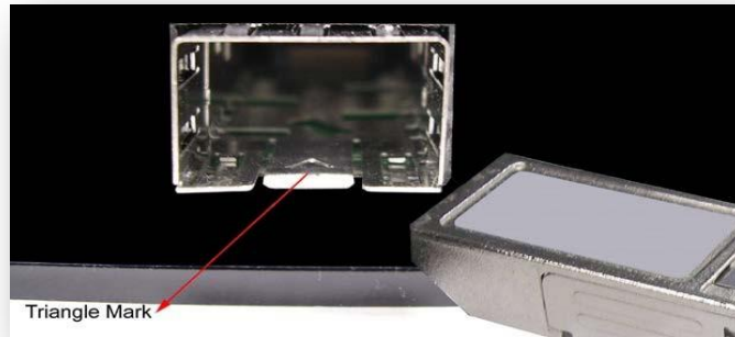
Figure 2.9 Transceiver to the SFP Module
