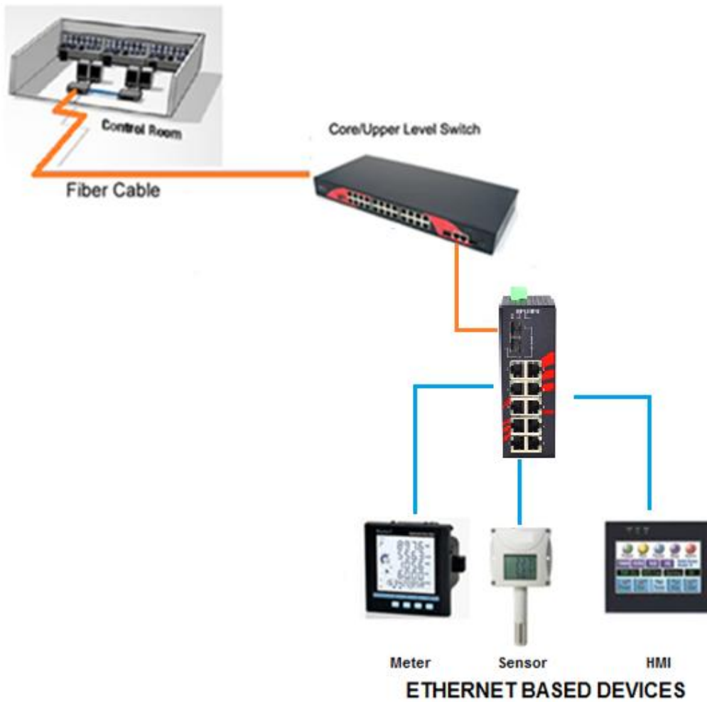
Figure 5.1 Industrial Ethernet Switch Application Reference
