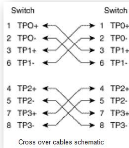
Figure 2.8 - Crossover Cables Schematic
