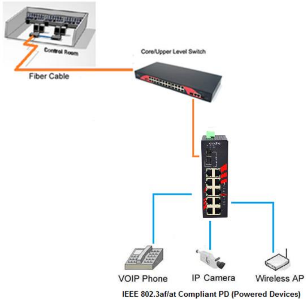
Figure 5.1 Industrial Ethernet Switch Application Reference
