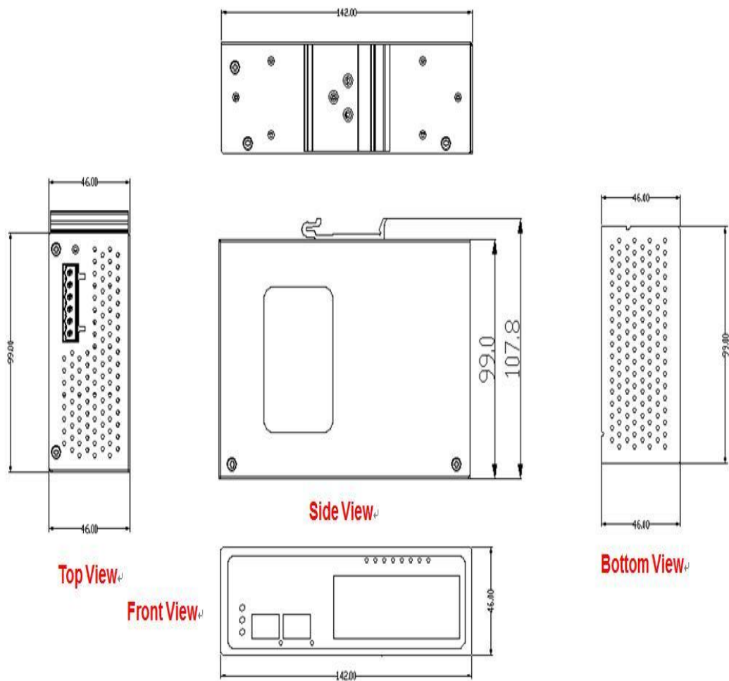
Figure 2.1 LNP-1002G-SFP-24 Series Physical Dimensions
