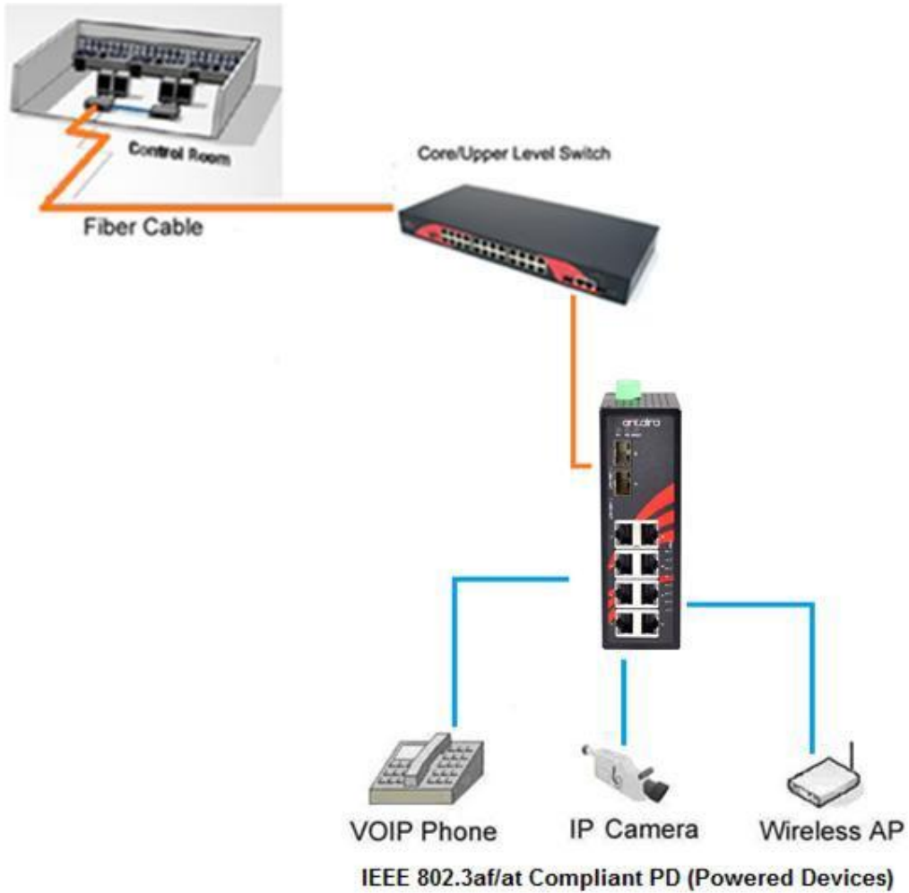
Figure 5.1 Industrial Ethernet Switch Application Reference
