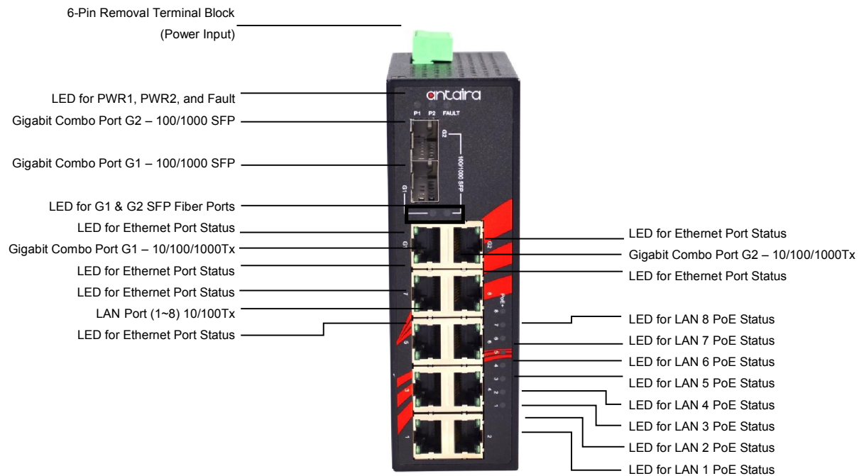
Figure 2.2 - Front Panel of LNP-1002C-SFP Series
