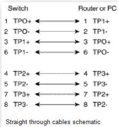
Figure 2.7 - Straight-Through Cables Schematic
