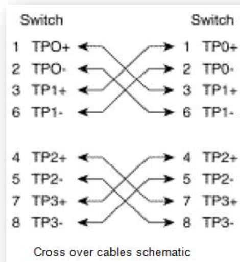
Figure 2.8 - Crossover Cables Schematic
