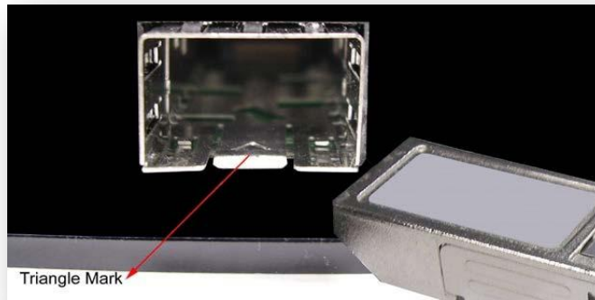
Figure 2.9 - Transceiver to the SFP Module
