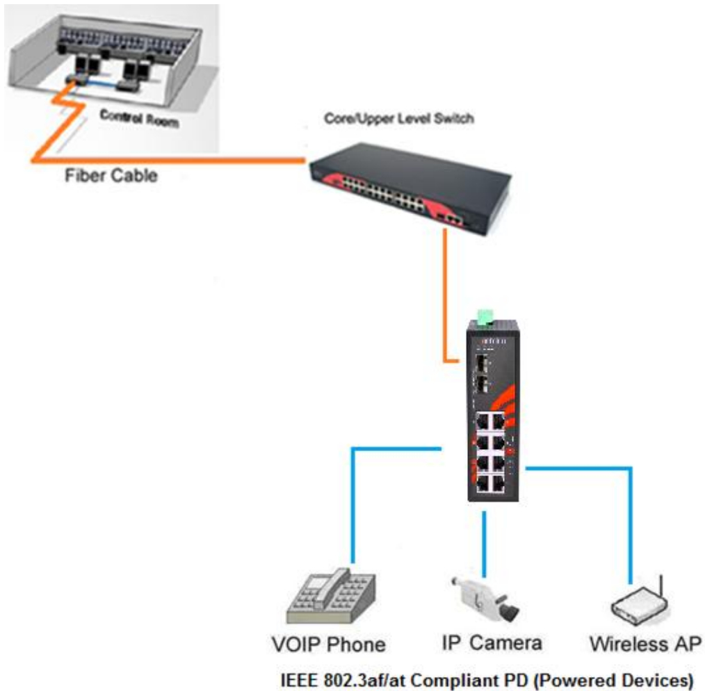
Figure 5.1 Industrial PoE Ethernet Switch Application Reference
