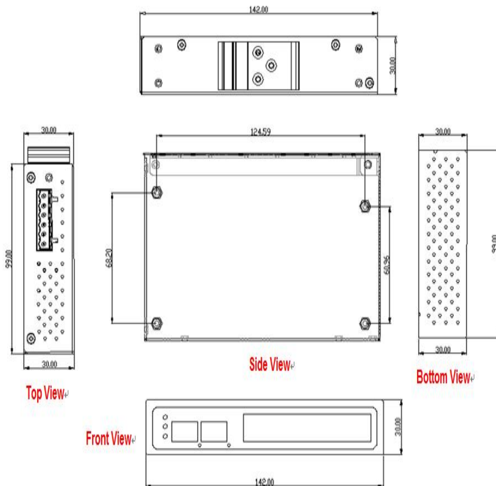
Figure 2.1 LNP-0702C-SFP Series Physical Dimensions
