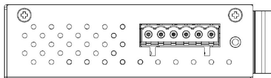
Figure 2.3 - Top Panel View of LNP-0702C-SFP Series
