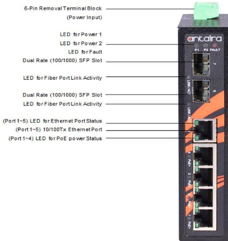
Figure 2.2 - The Front Panel of LNP-0702C-SFP Series
