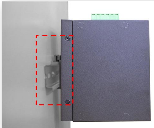
Figure 3.3 Stable the Switch on DIN-Rail
