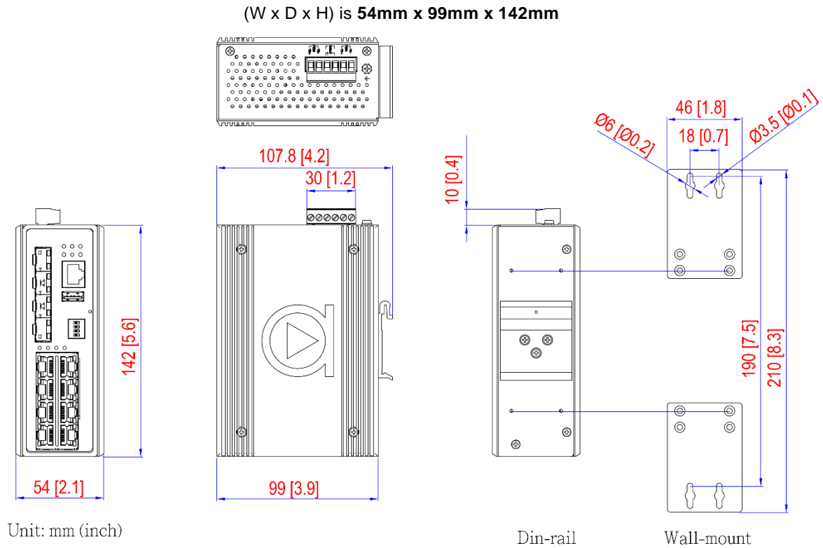
Figure 2.1 LMP-1204G-SFP-bt-24 Series Physical Dimensions
