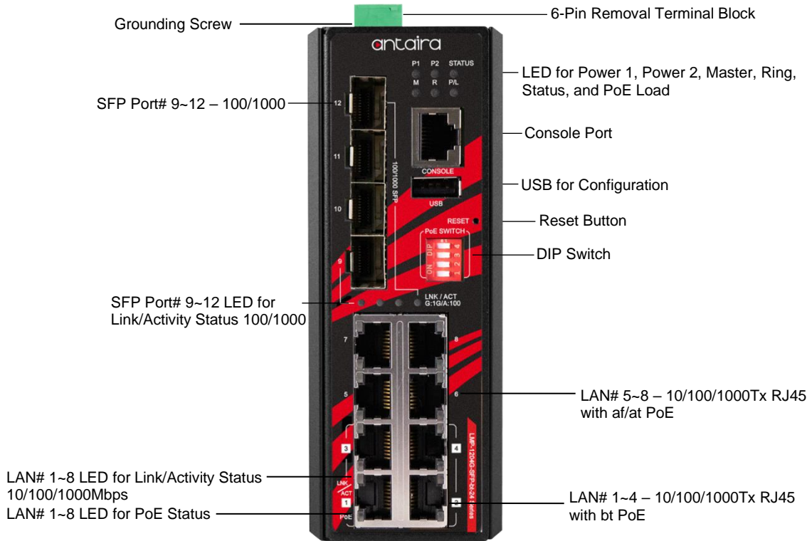
Figure 2.2 - The Front Panel of LMP-1204G-SFP-bt-24 Series
