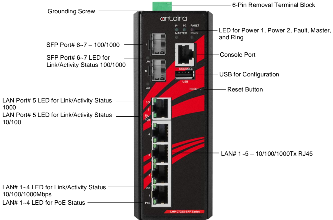
Figure 2.2 - The Front Panel of LMP-0702G-SFP-V2 Series
