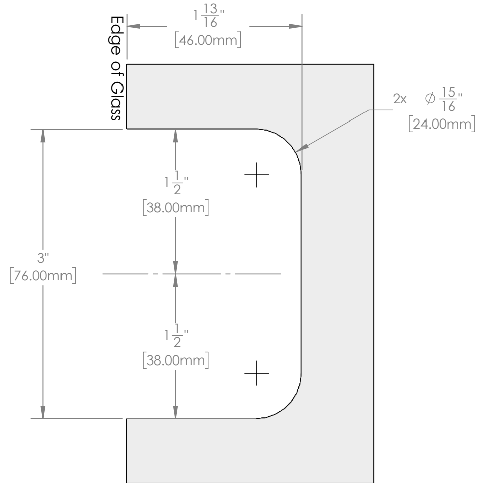
Rectangular Cutout Option
