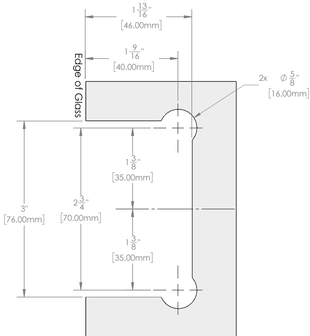
Mouse Ear Cutout Option
