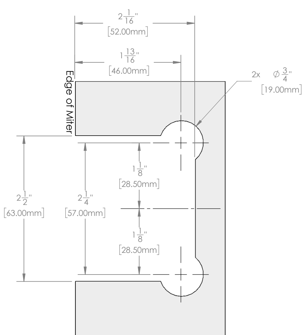
Mitered Fixed Panel Template
