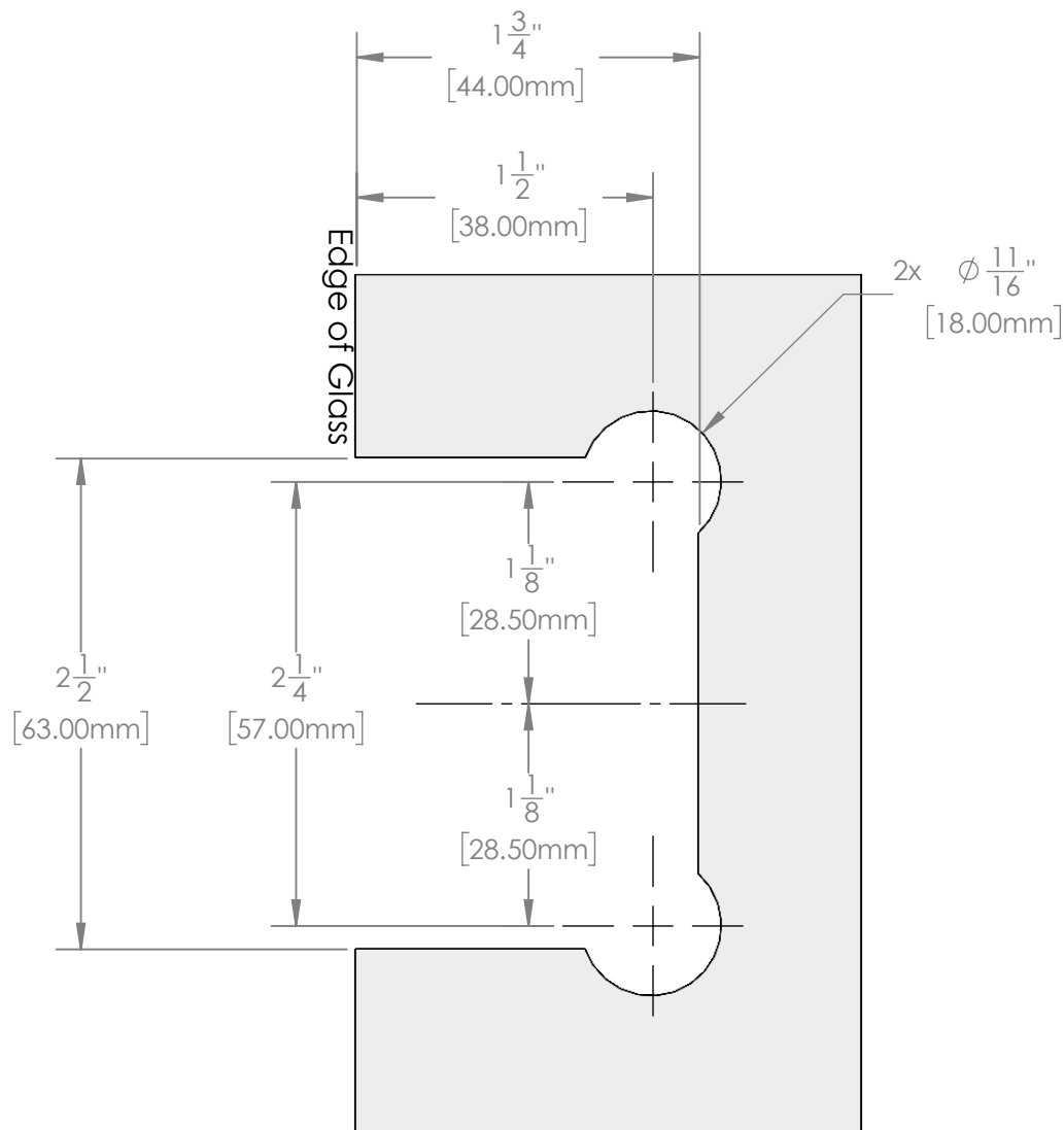
Square Cut Template
