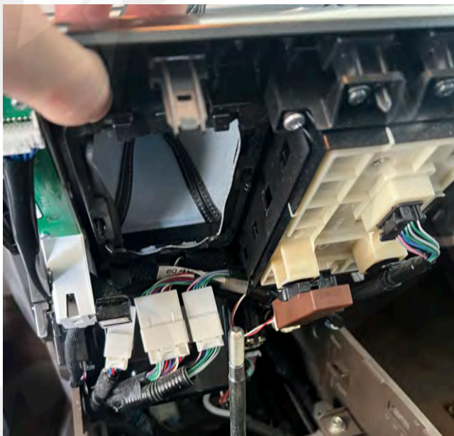
7. Disconnect (5) plugs. Two that are not shown are connected to the AUX / USB hub. NOTE: with the USB hub disconnected, 'AUX' will not display as a source choice!
