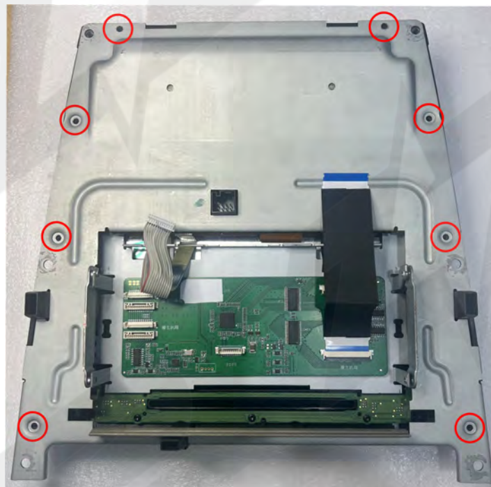
9. Replace the backing plate (removed on step 6) and replace all (8x) Torx screws.
