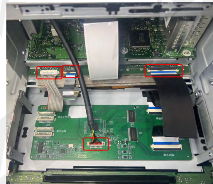
11. Connect the PCB Cable to the middle connector, paying careful attention to plug it in the proper orientation. Connect the lower black ribbon to the radio chassis from the provided PCB. Connect the remaining OE ribbons back to the radio chassis connectors.
