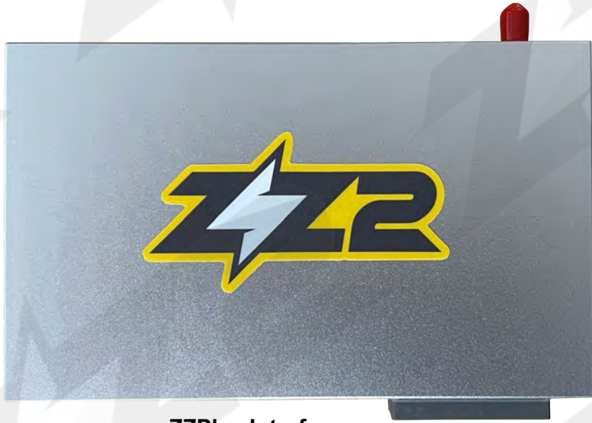
ZZPlay Interface
