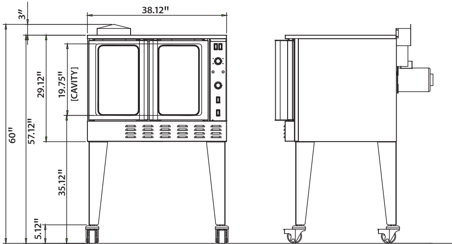
Single Oven with Leg and Caster Kit
