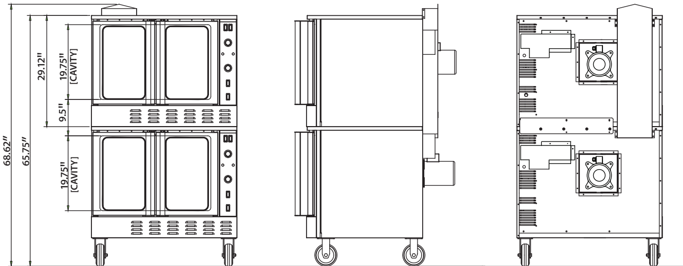
Dual Oven Configuration with Stacking Kit
