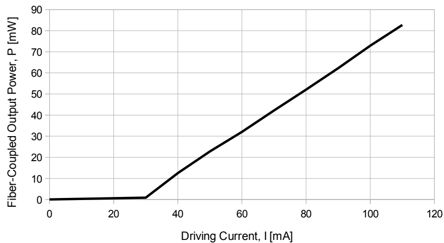
Fiber-coupled output power versus injection current 50 \mu m core diameter, NA 0.22
