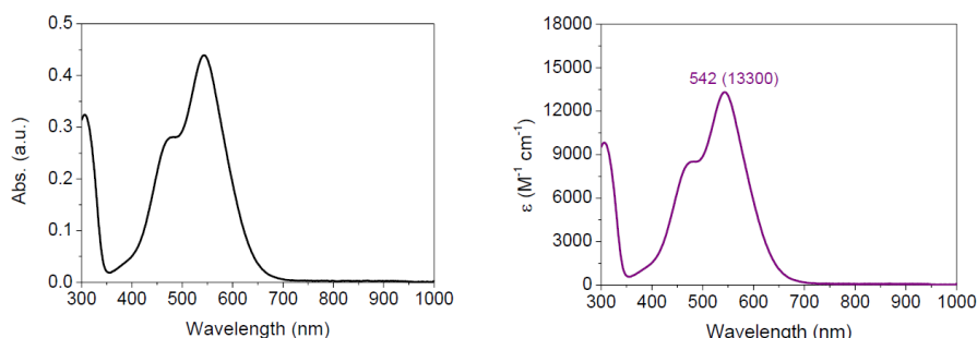
Figure 1 Absorption spectrum of water sample of reference (left) and batch produced (right)
