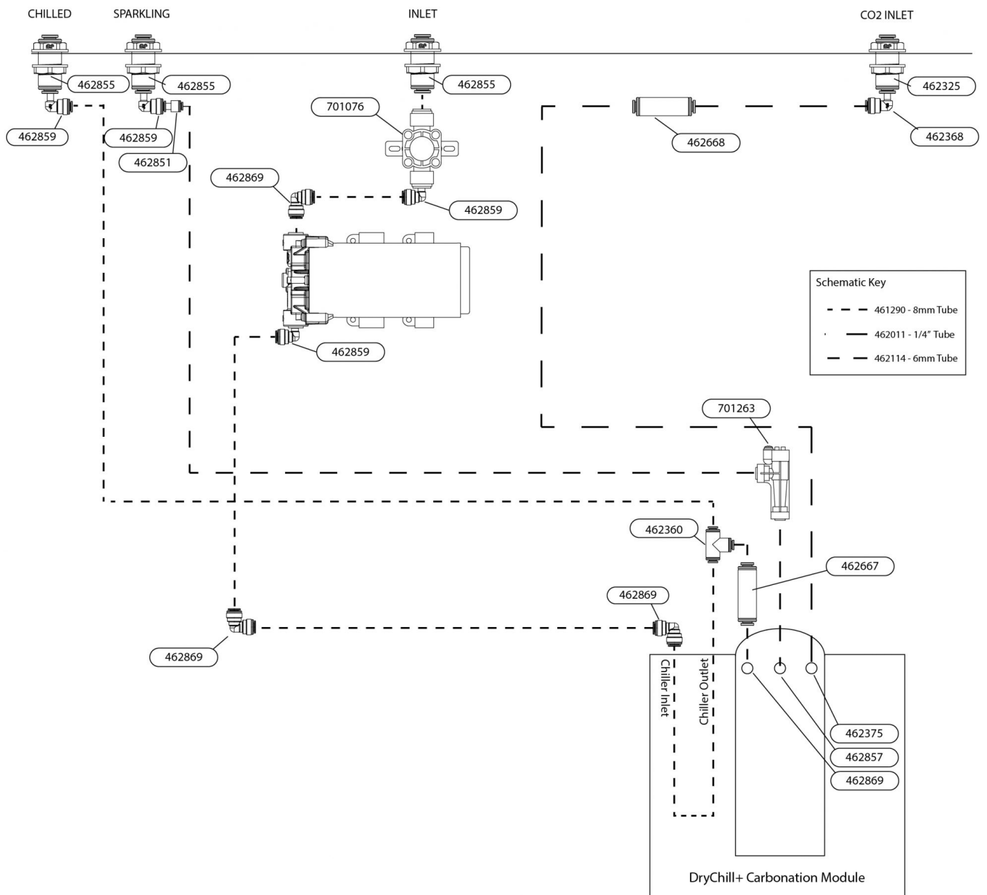
Water Pathway - Chilled, Ambient & Sparkling
