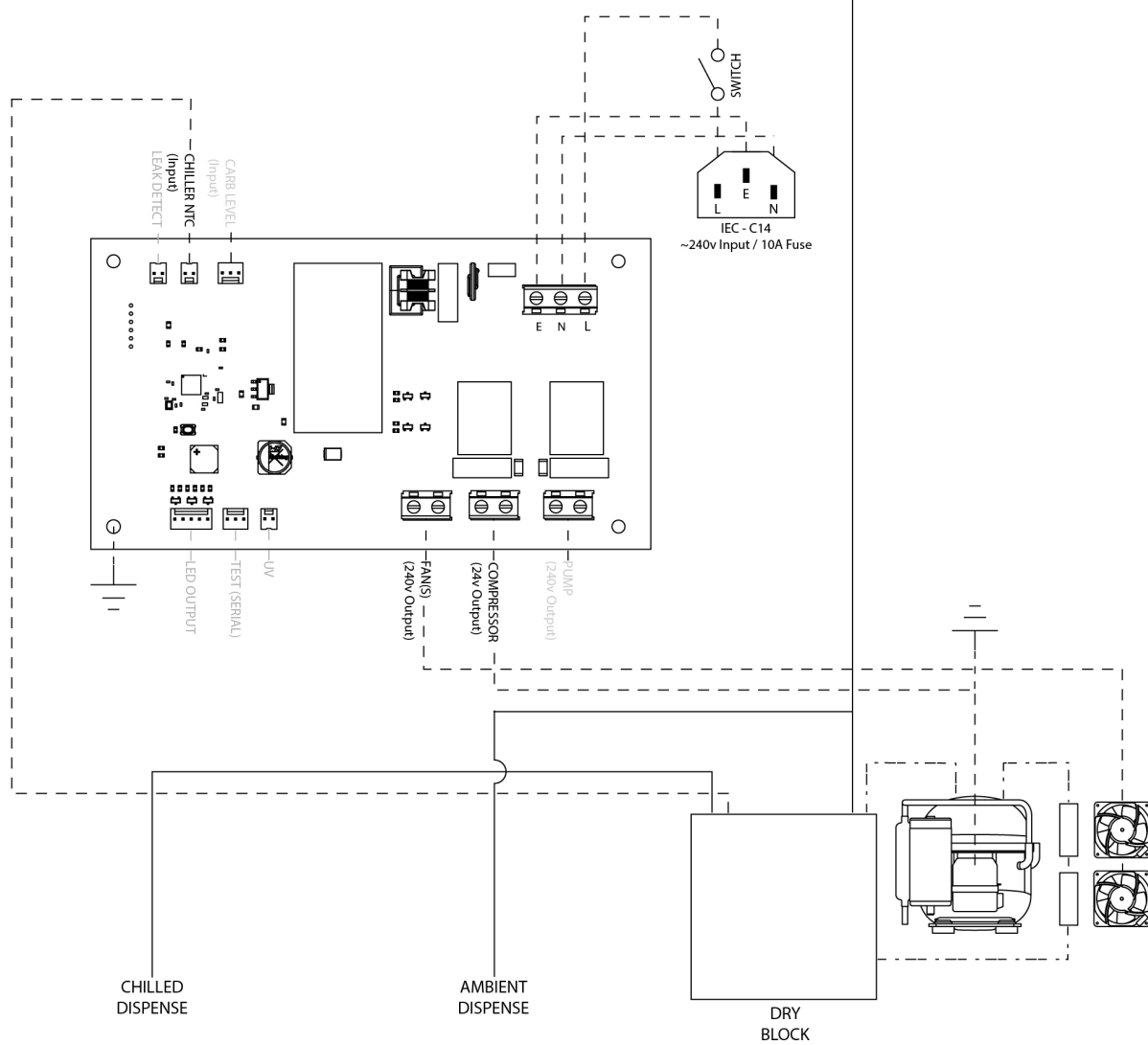
C2/C3 Chilled & Sparkling Circuit Schematic
