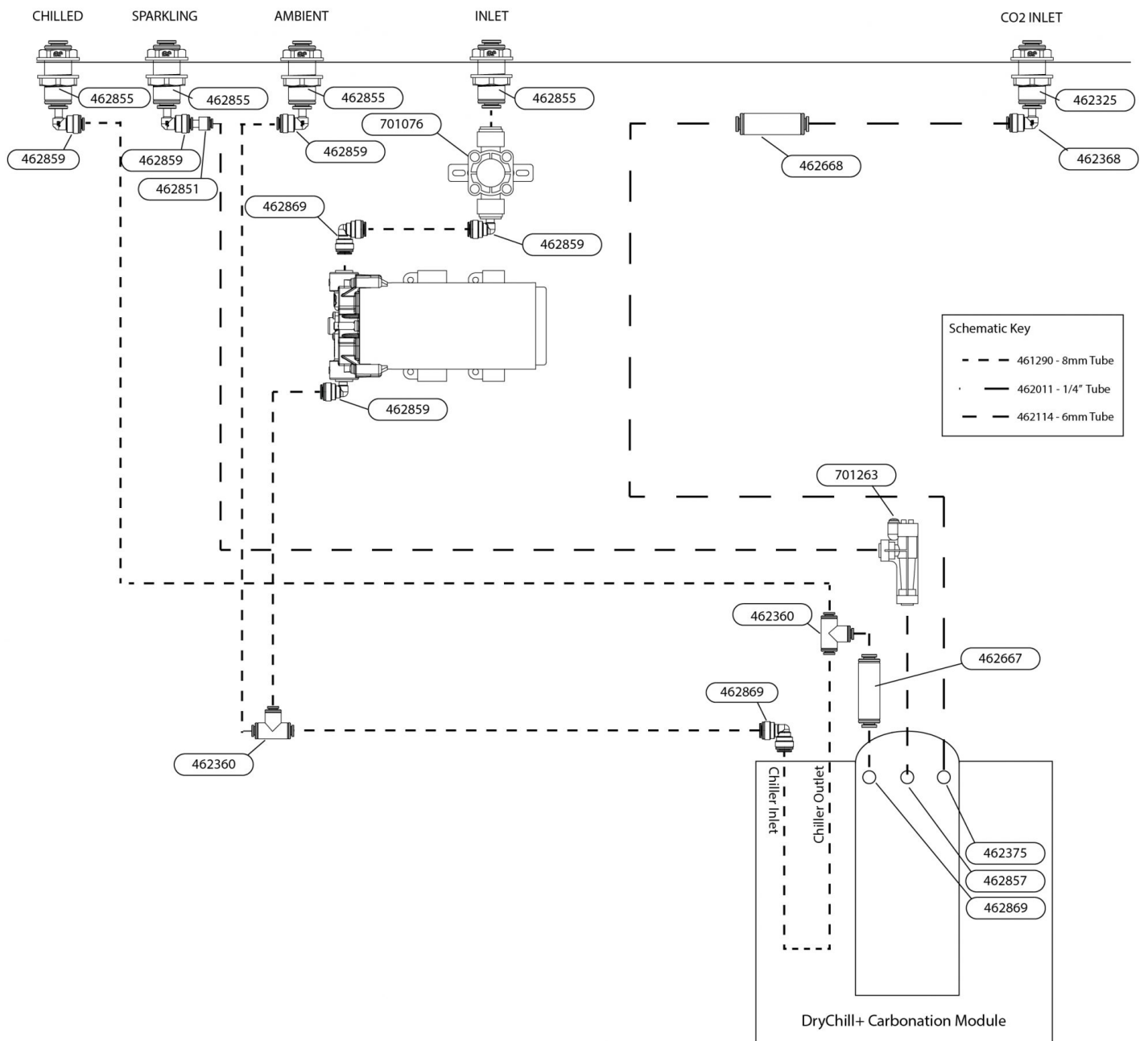
C2/C3 Chilled & Ambient Circuit Schematic
