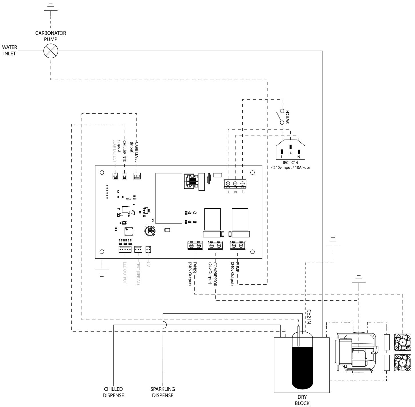
C2/C3 Chilled, Ambient & Sparkling Circuit Schematic
