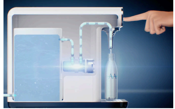
The Klaran Shield consists of small chamber through which the water flows from the Direct Chill Tank to the Tap. On its way the water is exposed with UVC LED wavelength radiation which is highly effective in destroying water-borne Bacteria and Viruses
