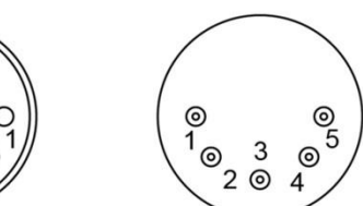
5 Pin XLR
