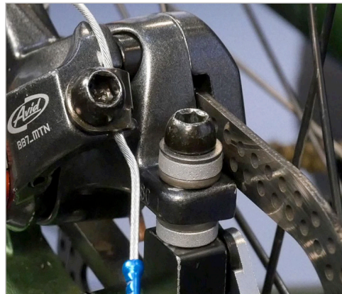
CALIPER WITH AVID CPS CONICAL WASHER SYSTEM
