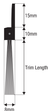
"H" PROFILE 180° STANDARD CARRIER
