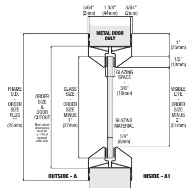
PROFILES AA A = Blind side
