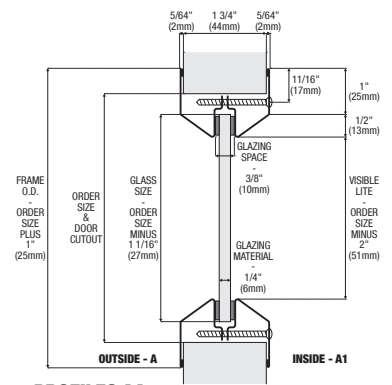
PROFILES AA1 A = Blind side A1 = Screw hole side
