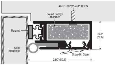
3708AA Concealed fixing magnetic frame seal included in acoustic tests up to 53 STC. With snap on cover. For use with steel doors or timber doors with steel strip (by others). 3708AA Anodised aluminium
