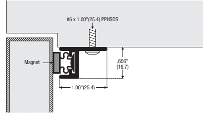
370A Surface fixing magnetic frame seal. For use with steel doors or timber doors with steel strip (by others). Available D finish to order. 370A Mill aluminium
