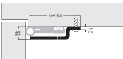
328SPB Strike plate bracket. Optional angle mounting bracket for 328 as shown and 475 frame seals to accommodate door closer brackets, panic bolt fittings or door co-ordinators. 152mm long. 328SPB Steel, grey painted
