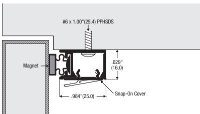
375AA Concealed fixing magnetic frame seal. For use with steel doors or timber doors with steel strip (by others). Available D finish to order. 375AA Anodised aluminium
