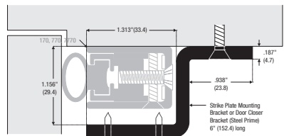
770SPB Strike plate bracket. Optional angle mounting bracket for 170, 770 and 7770 frame seals to accommodate door closer brackets, panic bolt fittings or door co-ordinators. 152mm long. 770SPB Steel, grey painted
