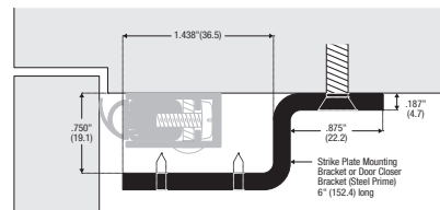
870SPB Strike plate bracket. Optional angle mounting bracket for 870 frame seal to accommodate door closer brackets, panic bolt fittings or door co-ordinators. 152mm long. 870SPB Steel, grey painted
