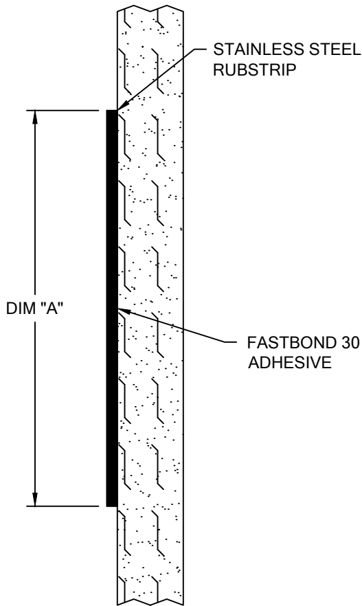
ADHESIVE INSTALLATION
