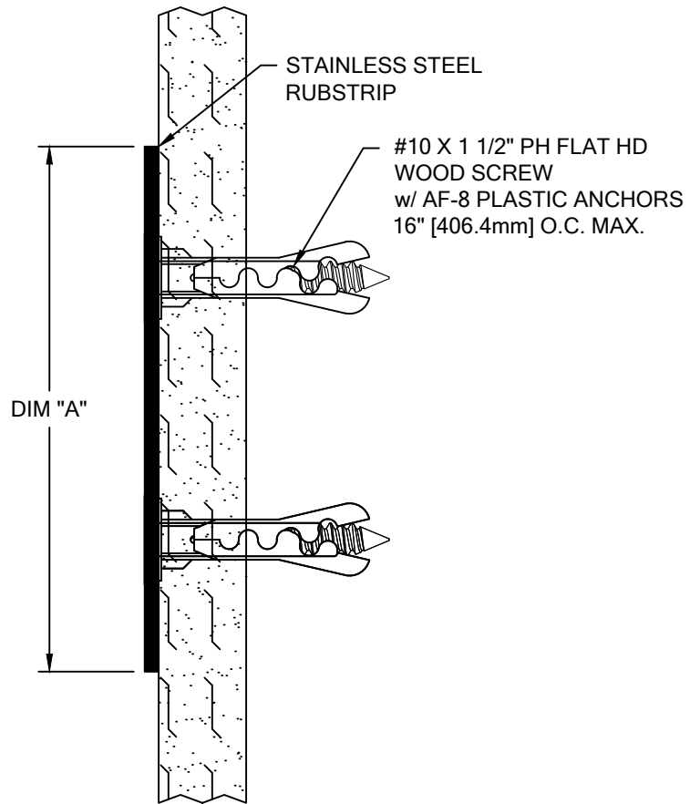
HARDWARE INSTALLATION
